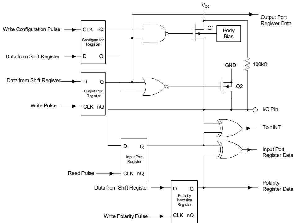
Figure 8. Block Diagram (Positive Logic)
