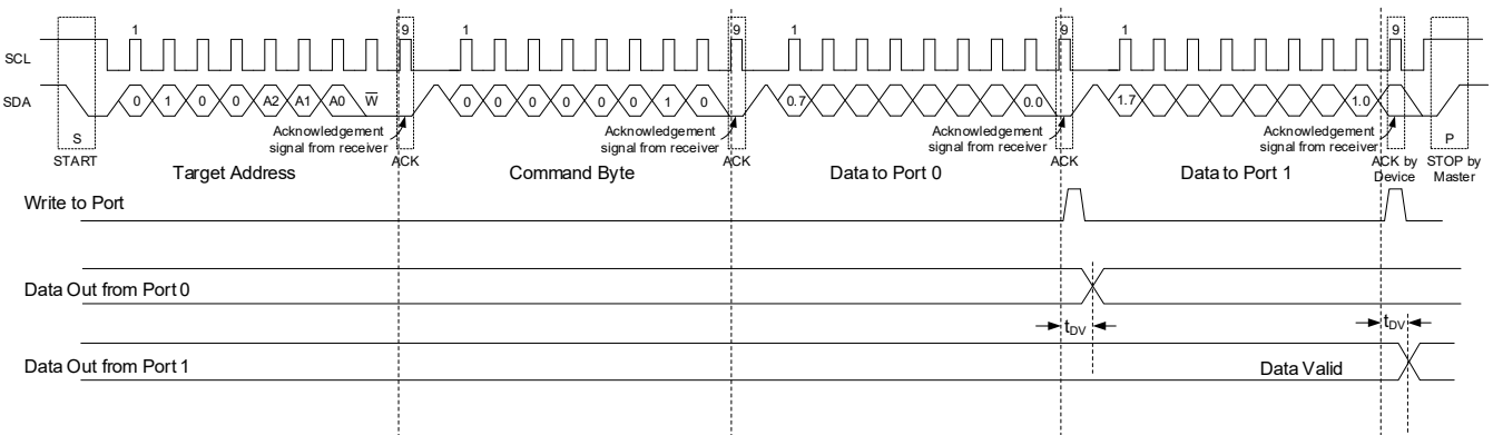
Figure 14. Write to Output Port 0 Register
