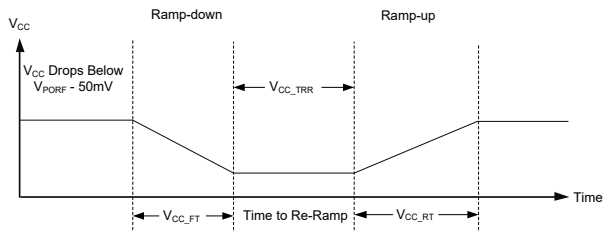
Figure 22. V CC Lowered below the POR Threshold, then Ramped Back
