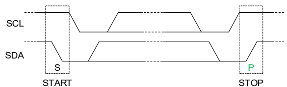
Figure 10. I 2 C Bus in START and STOP Conditions
