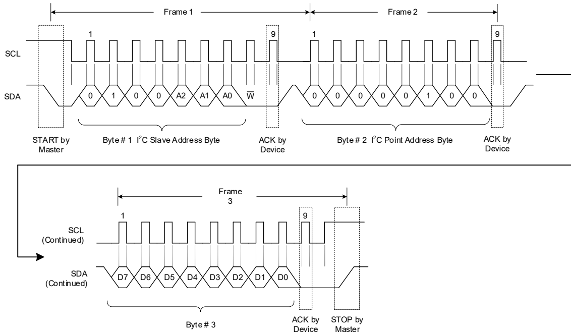
Figure 13. Write to the Polarity Inversion Port 0 Register
