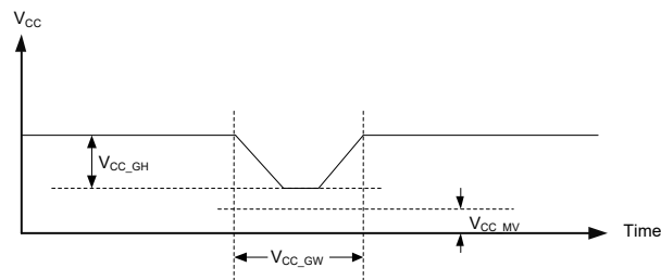
Figure 23. Width, Height and Minimum Voltage of Glitch
