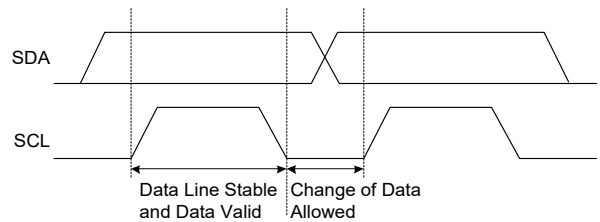
Figure 11. Bit Transfer
