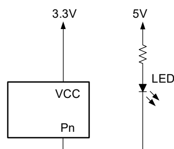
Figure 21. Device Supplied by Lower Voltage
