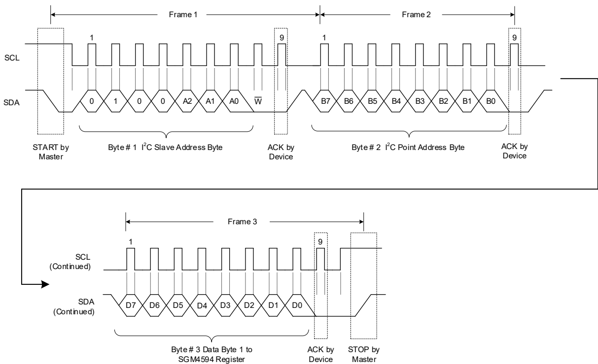
Figure 12. Write to Register
