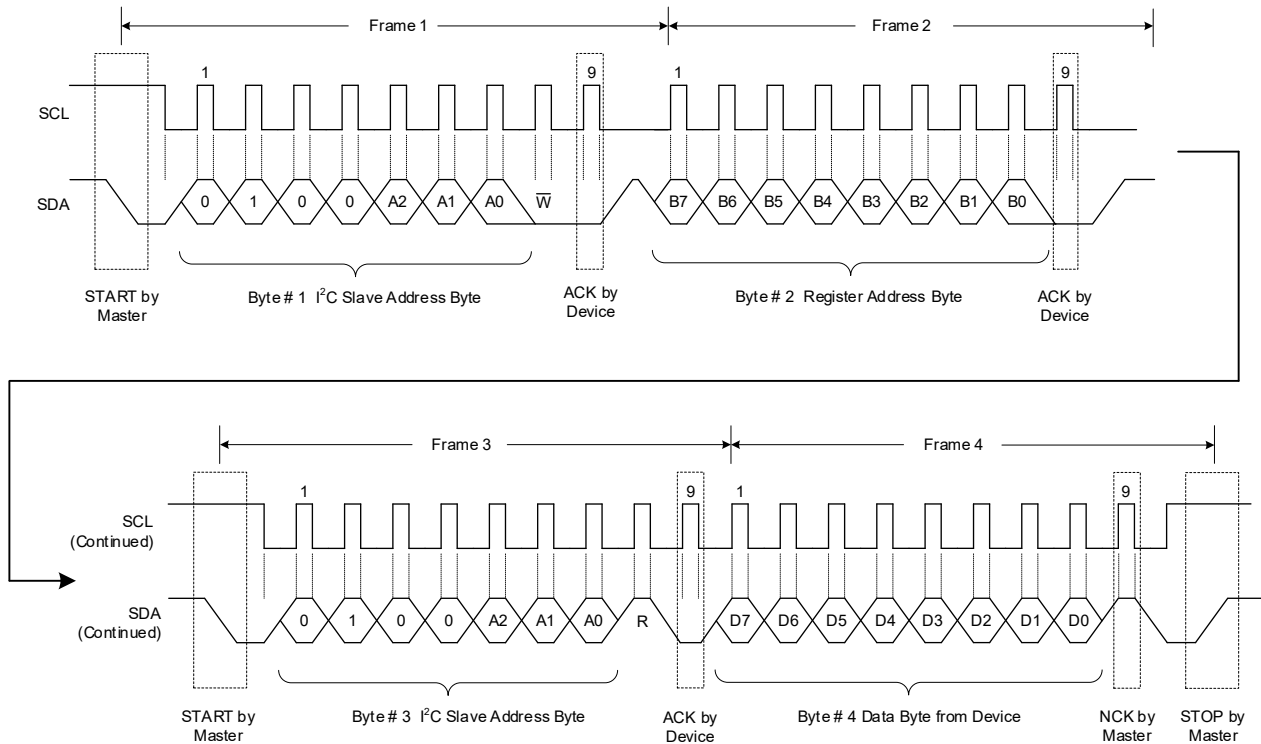
Figure 15. Read from Register
