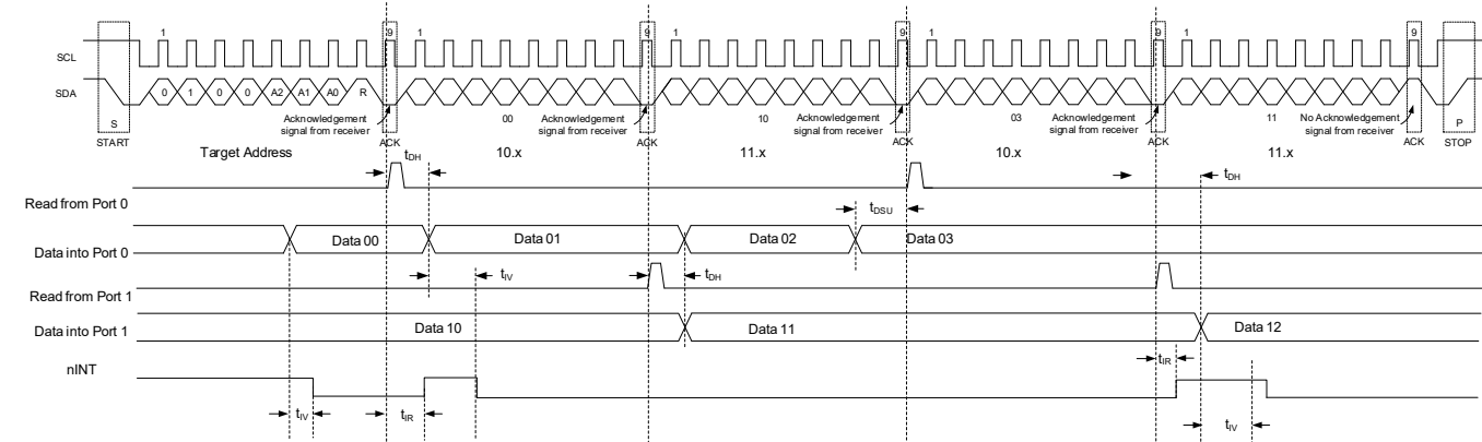
Figure 16. Scenario 1 of Read Input Port Register
