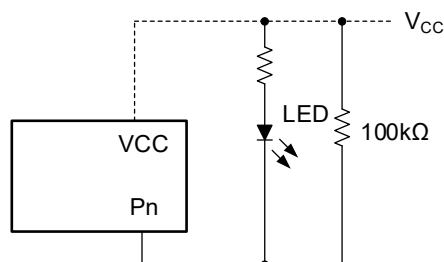
Figure 20. High-Value Resistor in Parallel with LED
