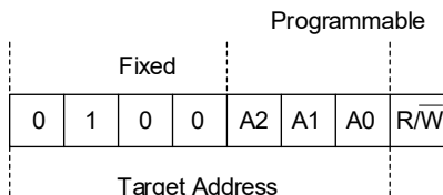
Figure 18. SGM4594 Address
