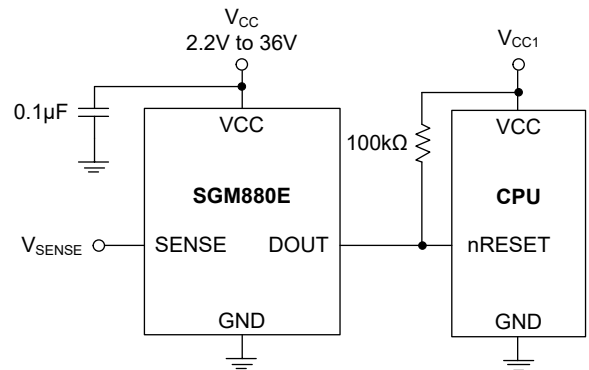
Figure 18. SGM880E Typical Application Circuit
