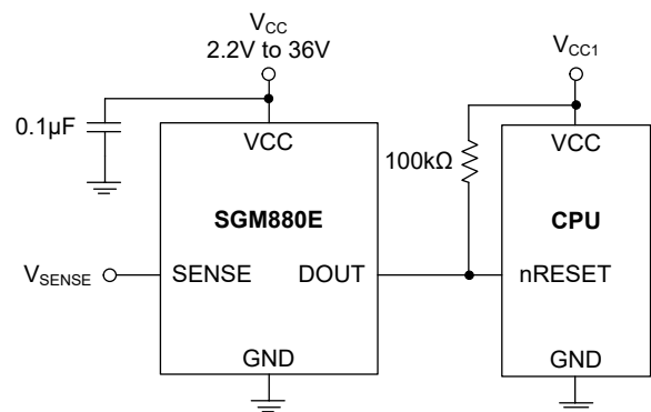
Figure 2. SGM880E Typical Application Circuit
