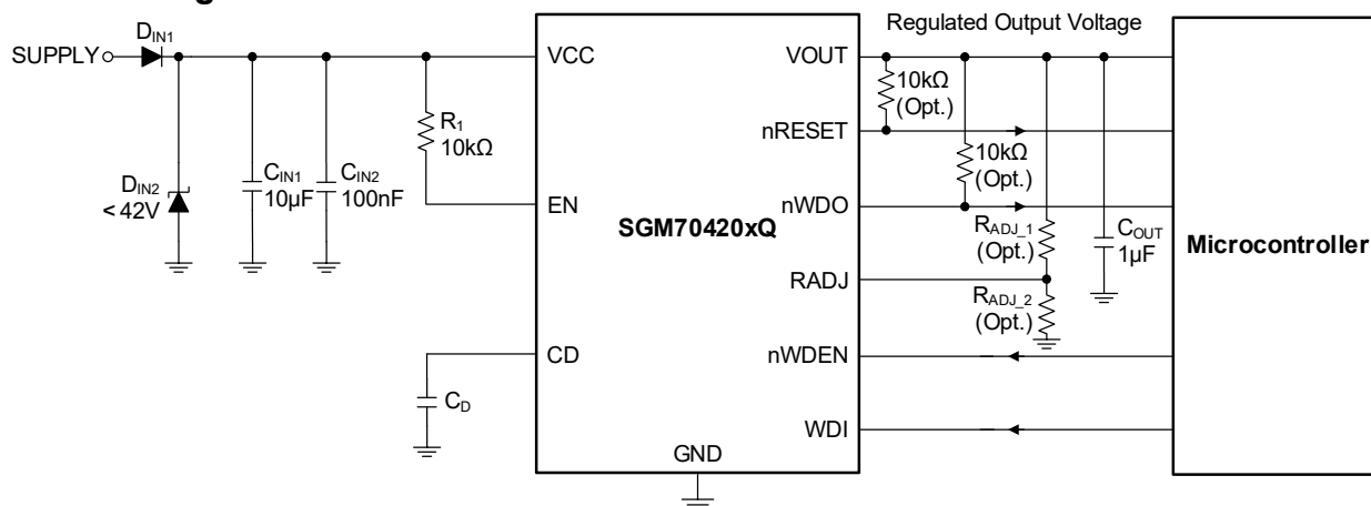
Figure 11. Application Diagram
