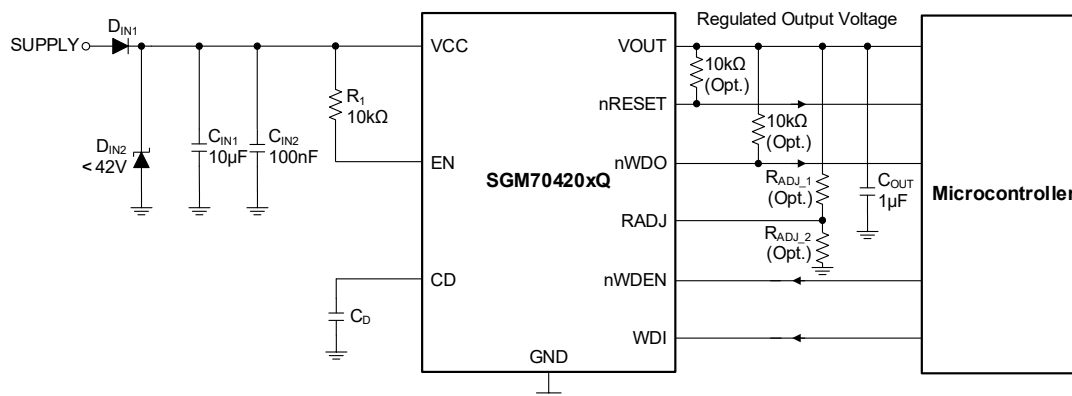
Figure 1. Simplified Schematic
