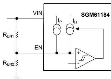
Figure 3. VIN UVLO Setting with a Resistor Divider
