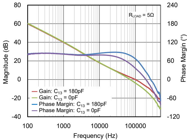
Loop Response
