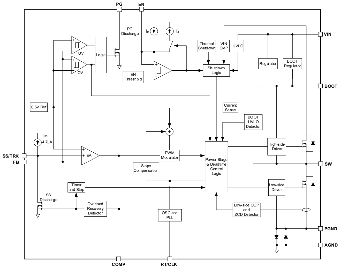
Figure 2. Block Diagram
