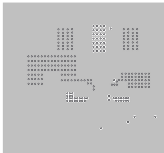
Figure 13. Mid Layer 1
