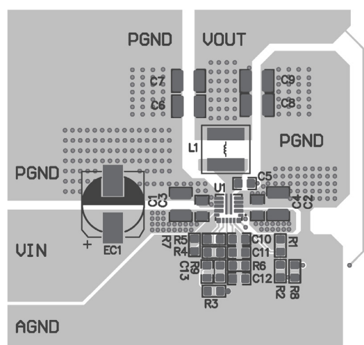
Figure 12. Top Layer
