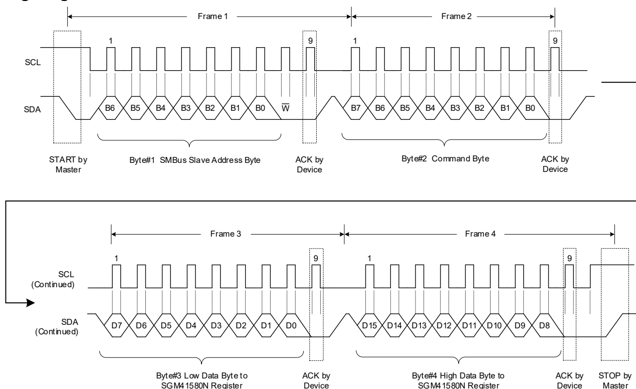
Figure 9. SMBus Write Timing
