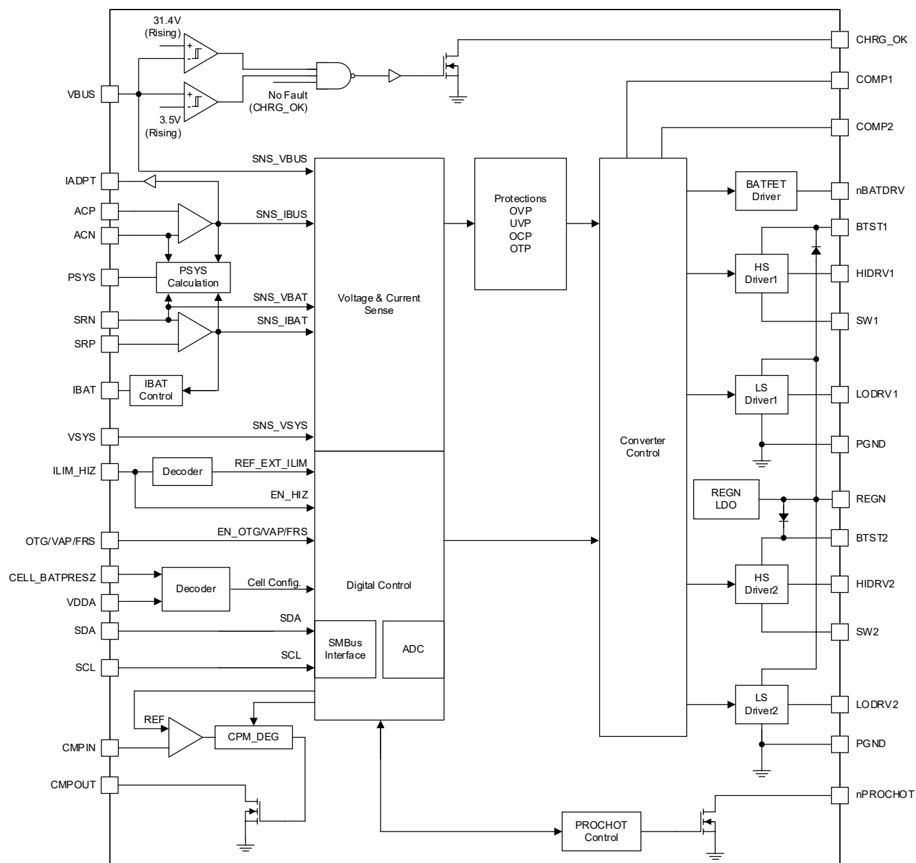
Figure 4. Block Diagram
