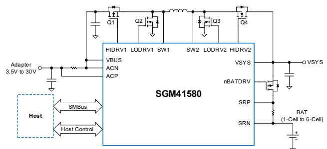
Figure 1. Simplified Schematic
