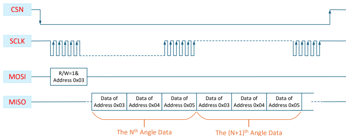
Figure 21. 4-Wire SPI Continuous Read Angle Data
