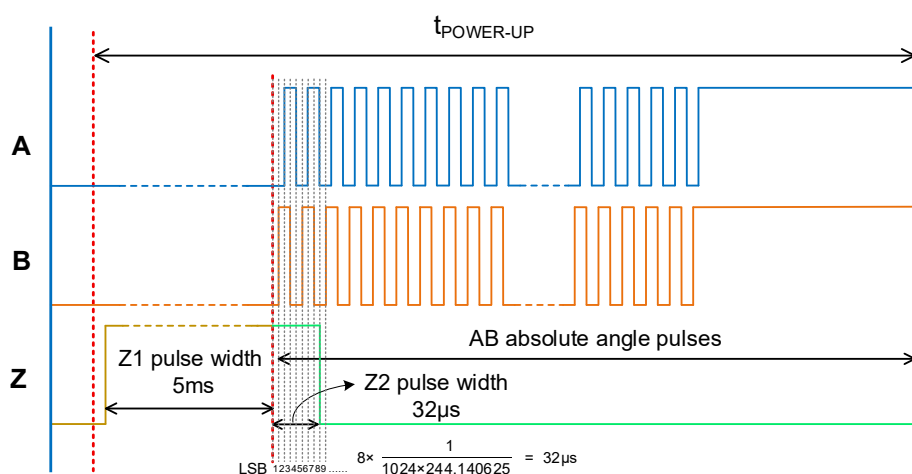
Figure 10. Power-Up Angular Output Signal of Pulse Sequence 2
