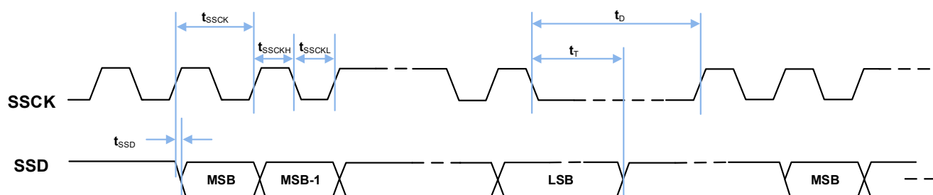
Figure 24. SSI Timing
