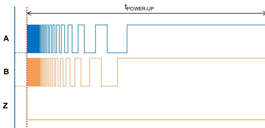
Figure 9. Power-Up Status Signal of Pulse Sequence 1
