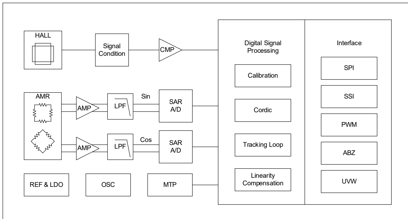
Figure 4. Block Diagram
