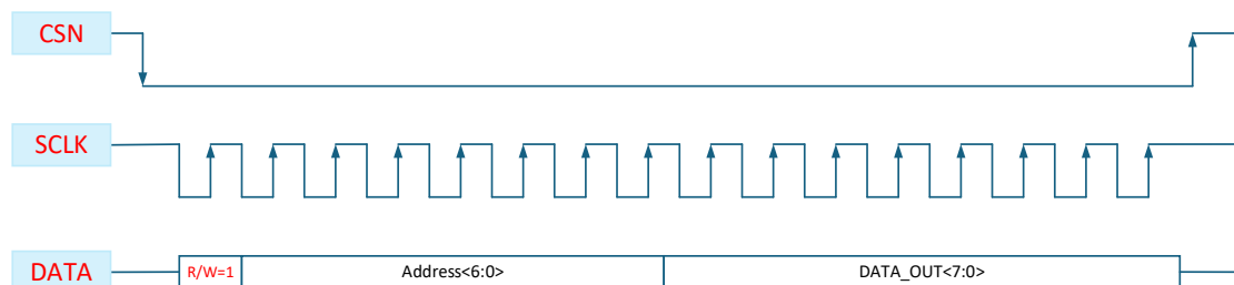
Figure 19. 3-Wire SPI Read Mode Timing Diagram
