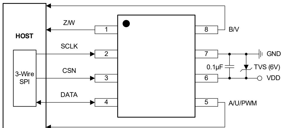
Figure 2. Application Circuit for ABZ/UVW/PWM/3-Wire SPI Modes (SOIC-8)
