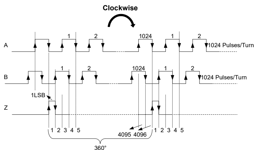
Figure 8. AB Signal Resolution is 1024 Pulses per Revolution in CW Mode during Clockwise Magnet Rotation
