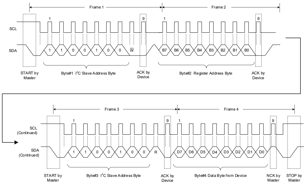
Figure 12. A Read Transaction
