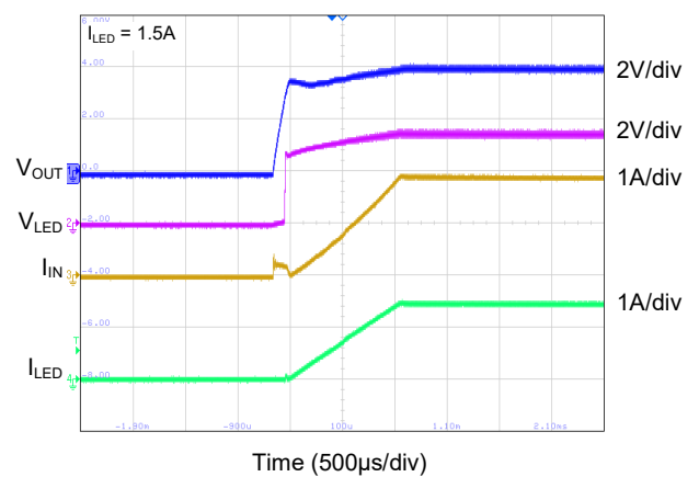
Flash Mode Start-Up
