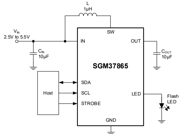
Figure 13. Typical Application Circuit
