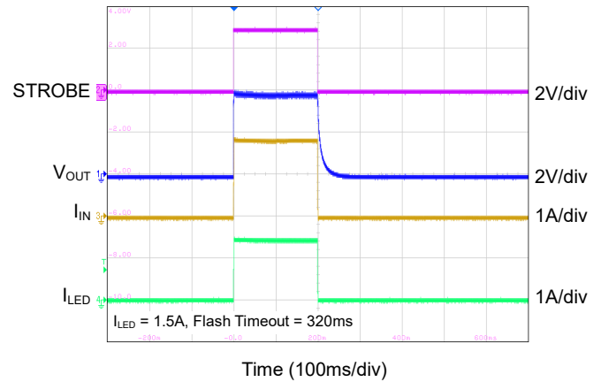
STROBE Level Triggered Flash
