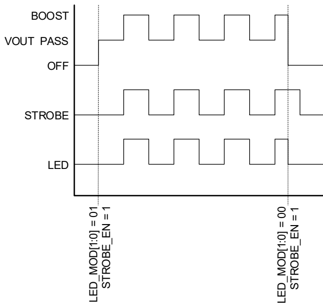
Figure 5. IR Mode with Boost
