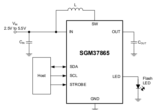
Figure 1. Simplified Schematic
