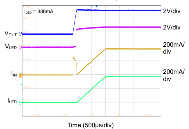
Torch Mode Start-Up
