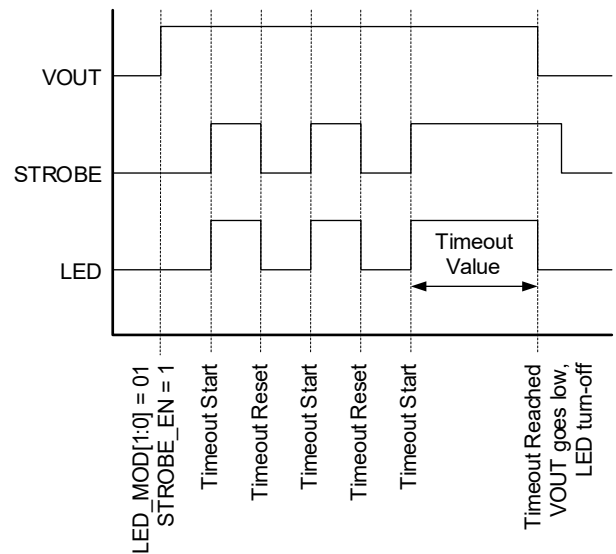
Figure 7. IR Mode Timeout
