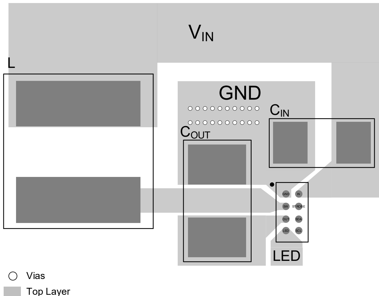
Figure 14. Layout Example
