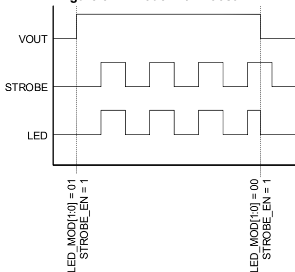
Figure 6. IR Mode Pass Only
