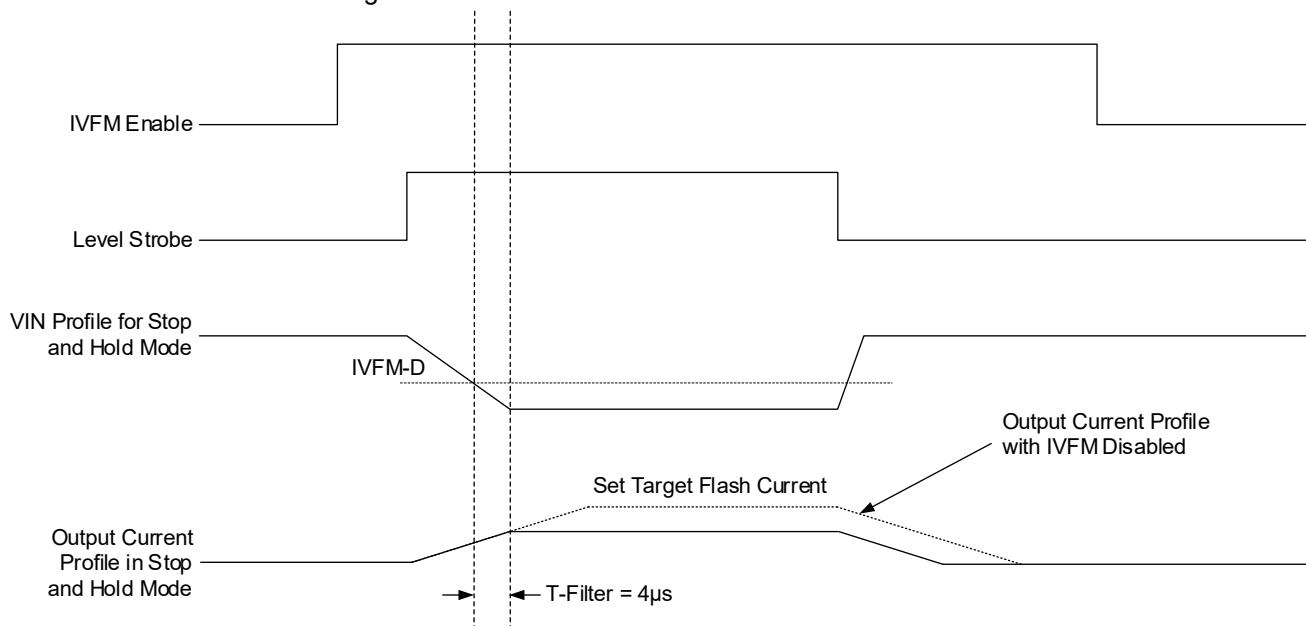
Figure 8. IVFM Mode
