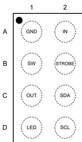
SGM37865 (TOP VIEW)
