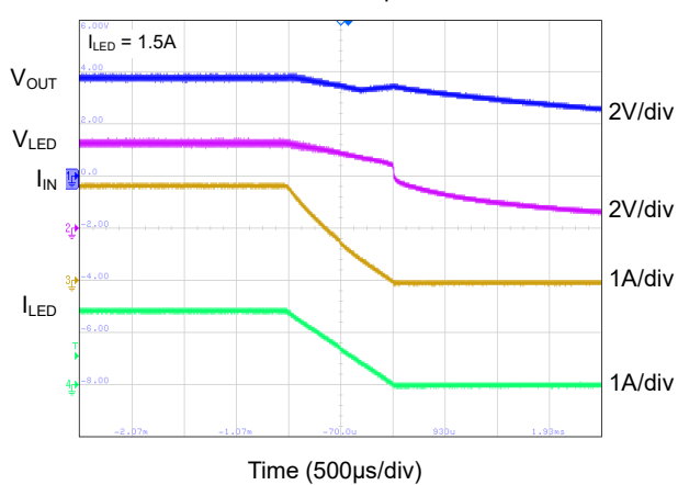
Flash Mode Ramp Down
