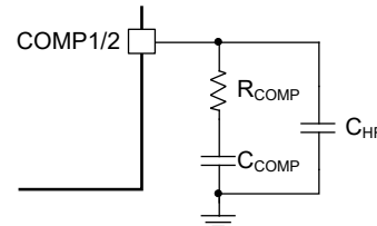
Figure 13. SGM64620Q External Compensation
