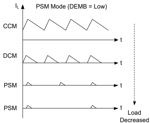
Figure 4. Converter Operation with PSM Enabled
