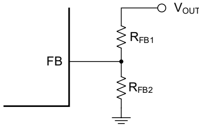
Figure 6. Output Voltage (V OUT1/2 ) Setting
