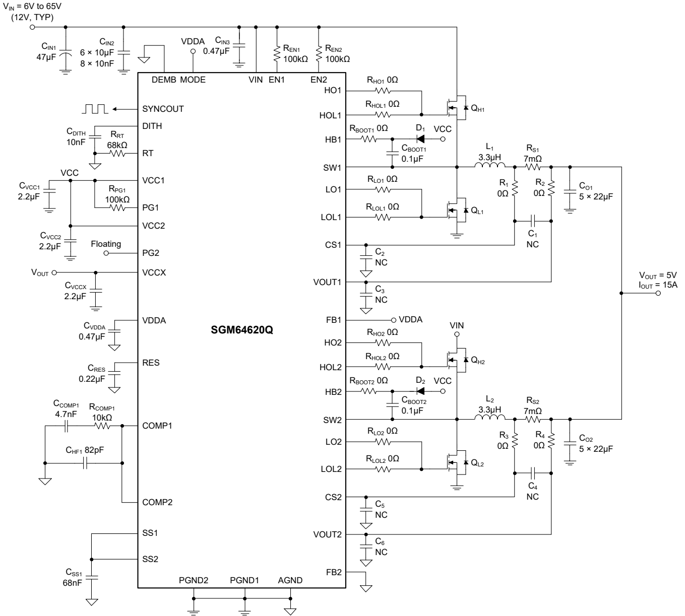
Figure 15. Application Circuit for Two-Phase 5V Single-Output with 400kHz
