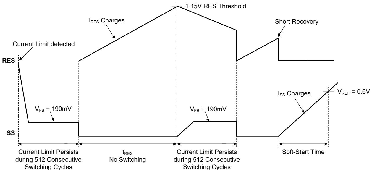
Figure 9. Hiccup Mode Timing Diagram
