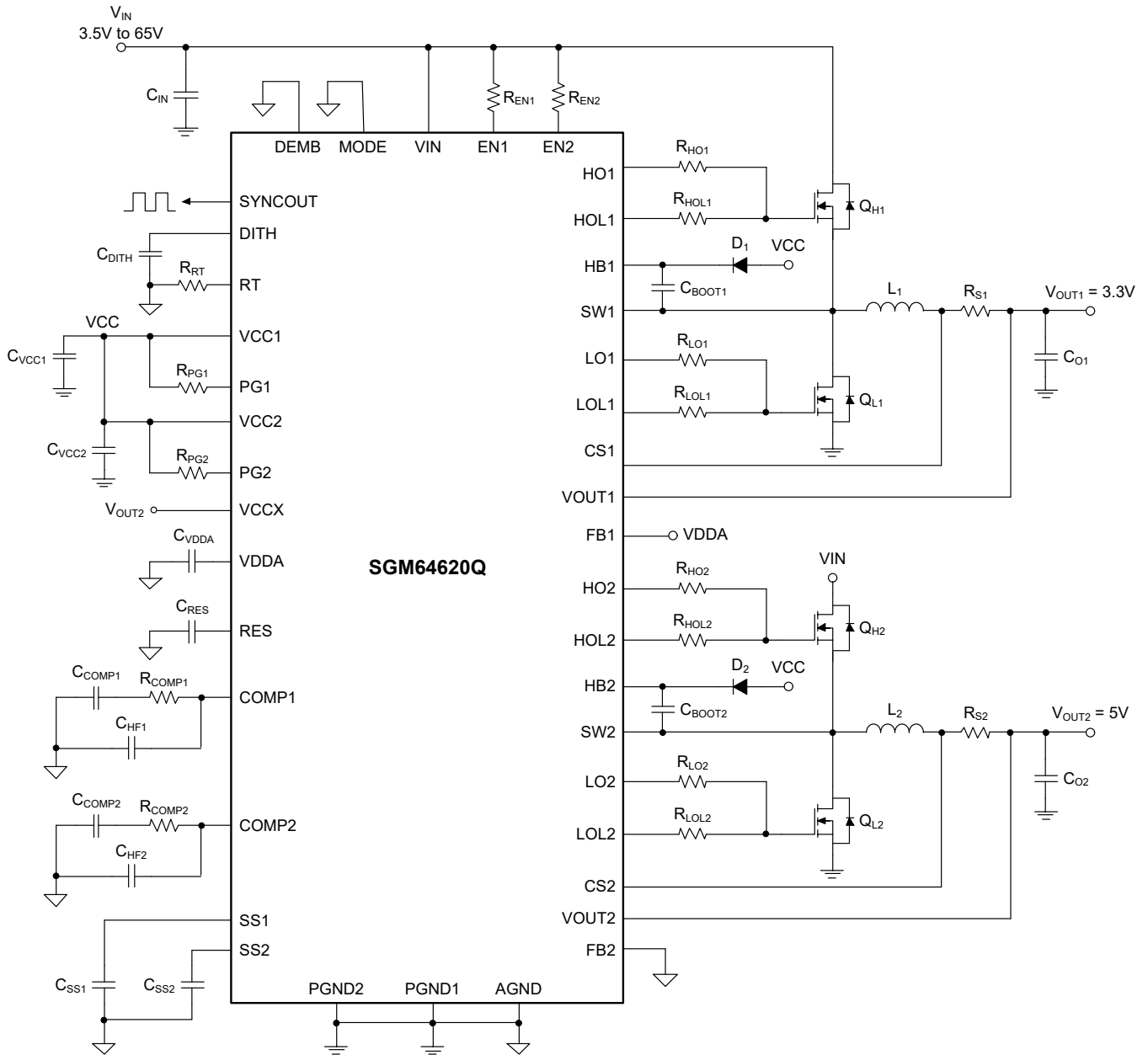
Figure 1. Simplified Schematic
