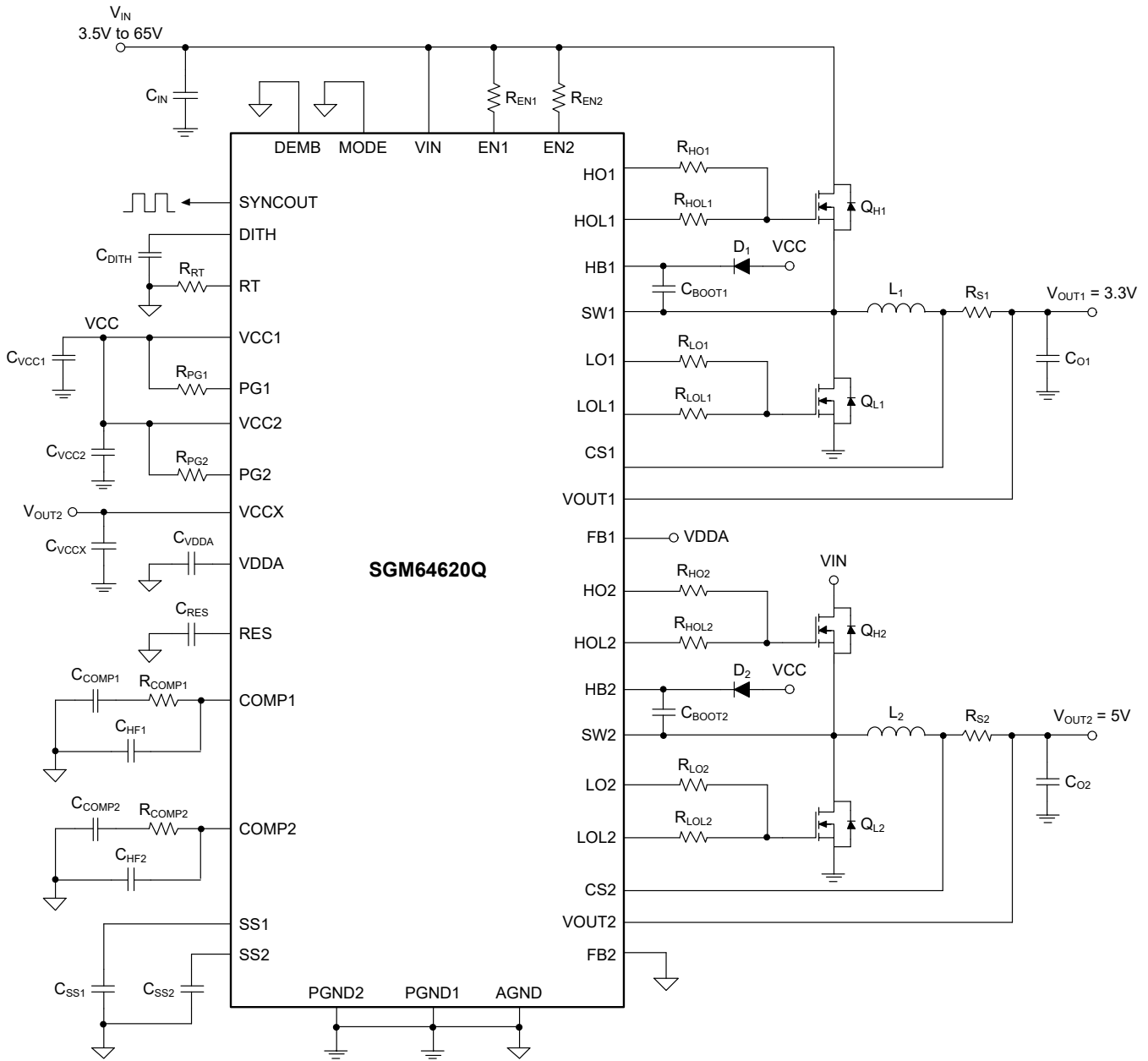
Figure 10. Independent Dual-Outputs Configurations Simplified Schematic
