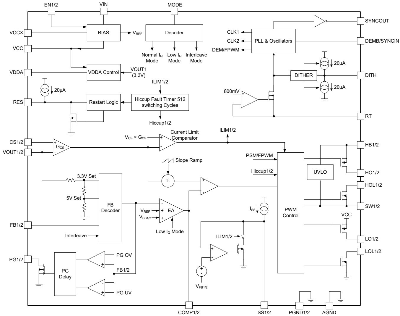
Figure 2. Block Diagram
