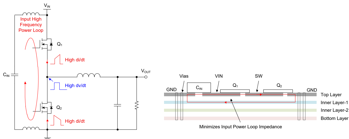
Figure 17. The Input Power Loop Layout Recommendation
