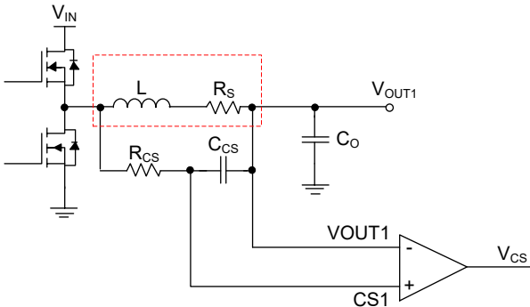
Figure 8. Inductor DCR Current Sensing Implementation
