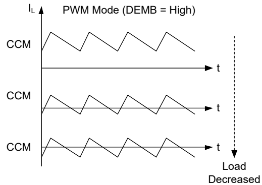
Figure 3. Converter Operation with Forced PWM (PSM Disabled)
