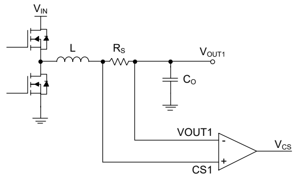
Figure 7. Shunt Current Sensing Implementation
