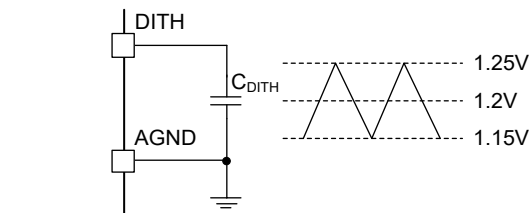
Figure 5. Switching Frequency Dithering
