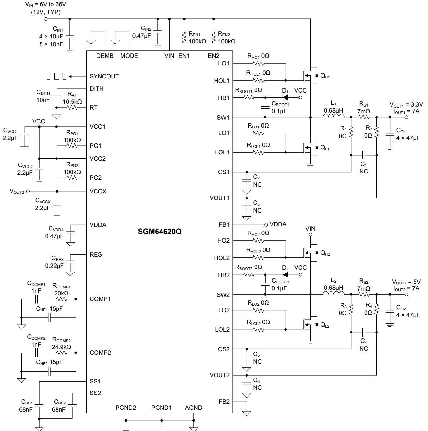
Figure 14. Application Circuit for 3.3V and 5V Dual-Output with 2.1MHz
