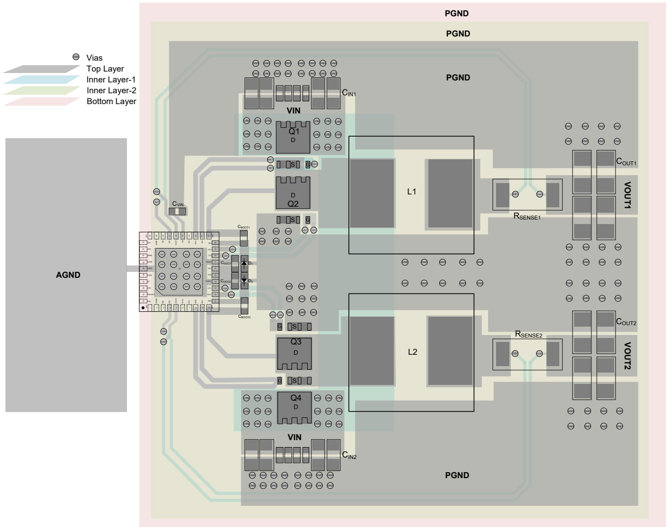
Figure 18. Layout Example
