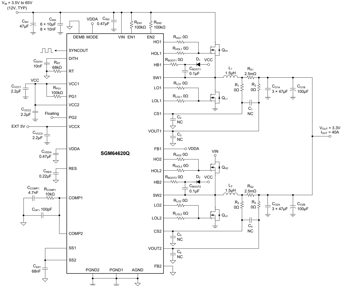
Figure 16. Application Circuit for Two-Phase 3.3V Single-Output with 400kHz
