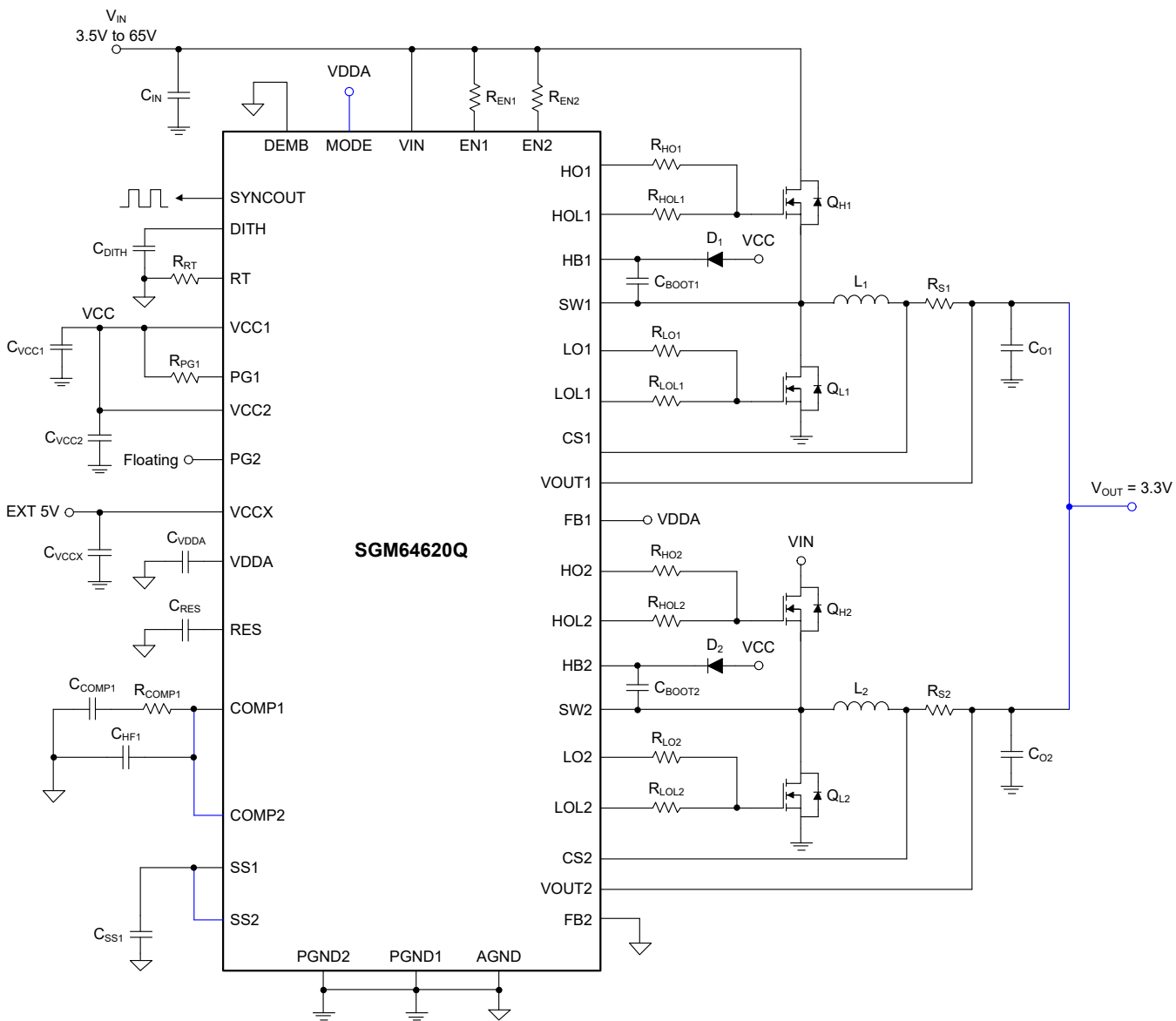
Figure 11. Single-Output Interleaved Configuration Simplified Schematic
