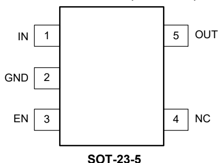
SGM2085L-FIXQ (TOP VIEW)
