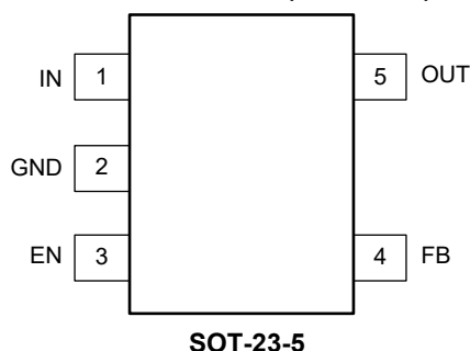
SGM2085L-ADJQ (TOP VIEW)
