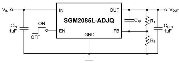
Figure 5. Adjustable Output Voltage Application
