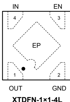
SGM2085L-FIXQ (TOP VIEW)
