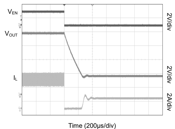
Shutdown Waveforms
