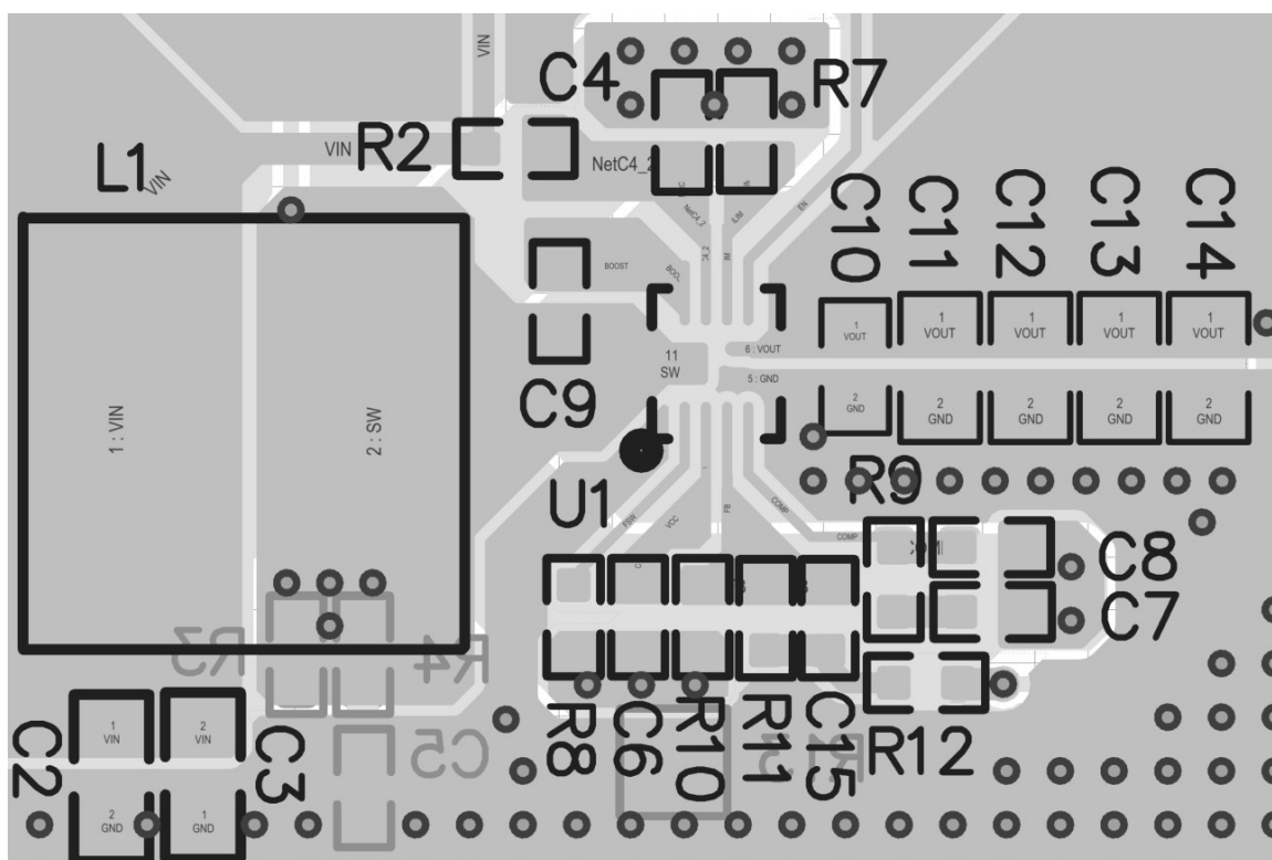
Figure 5. Layout Example
