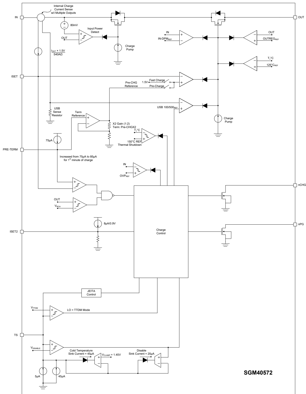
Figure 1. Block Diagram
