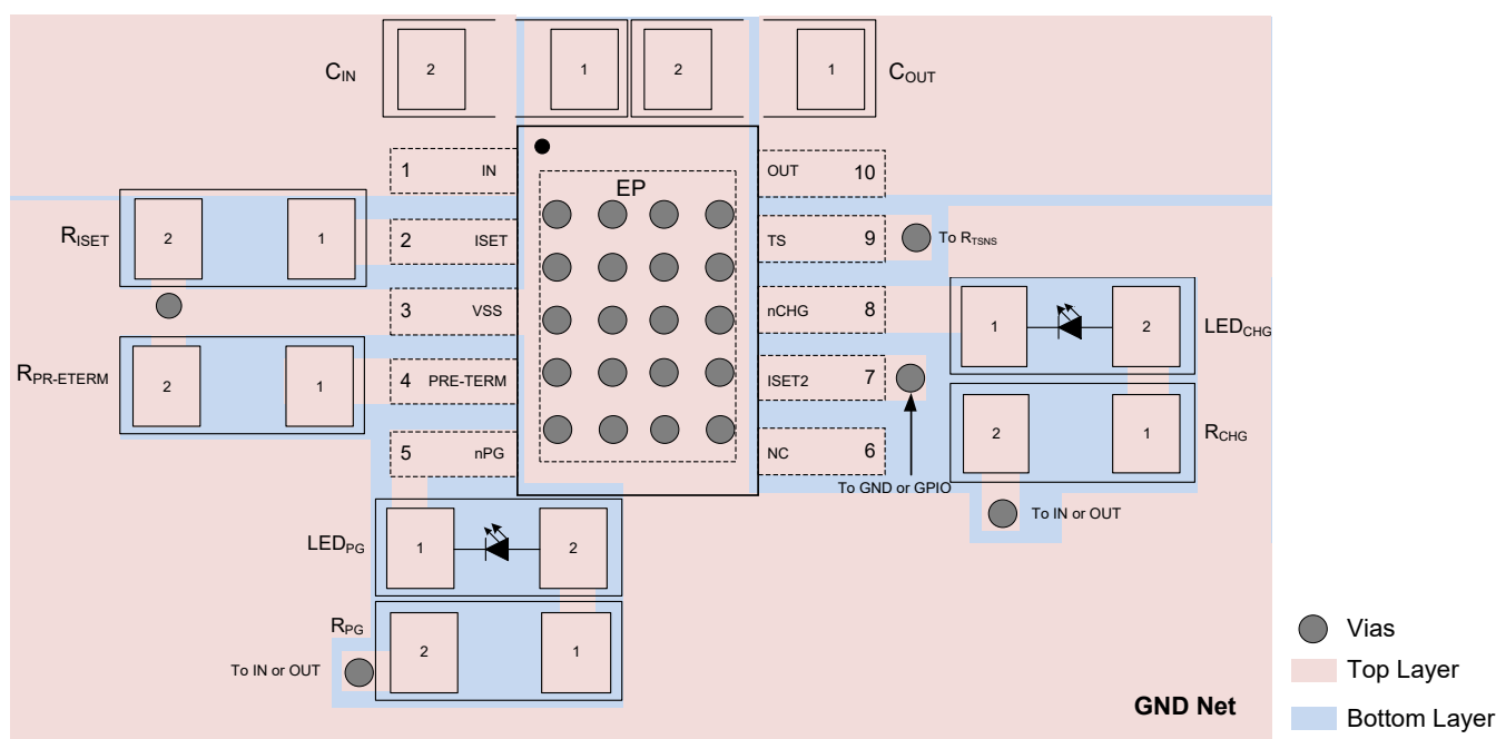
Figure 9. Board Layout
