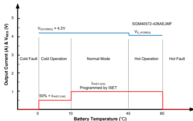
Figure 5. Operation vs. Battery Temperature
