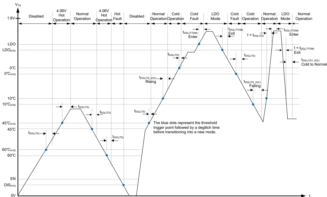
Figure 6. TS Battery Temperature Bias Threshold and Deglitch Timers
