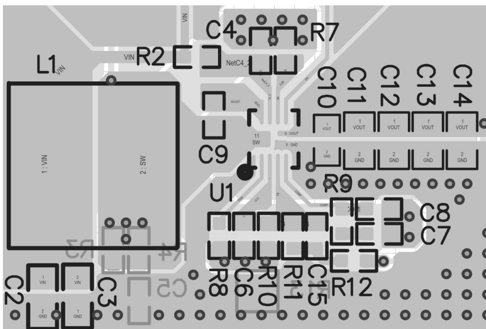
Figure 5. Layout Example
