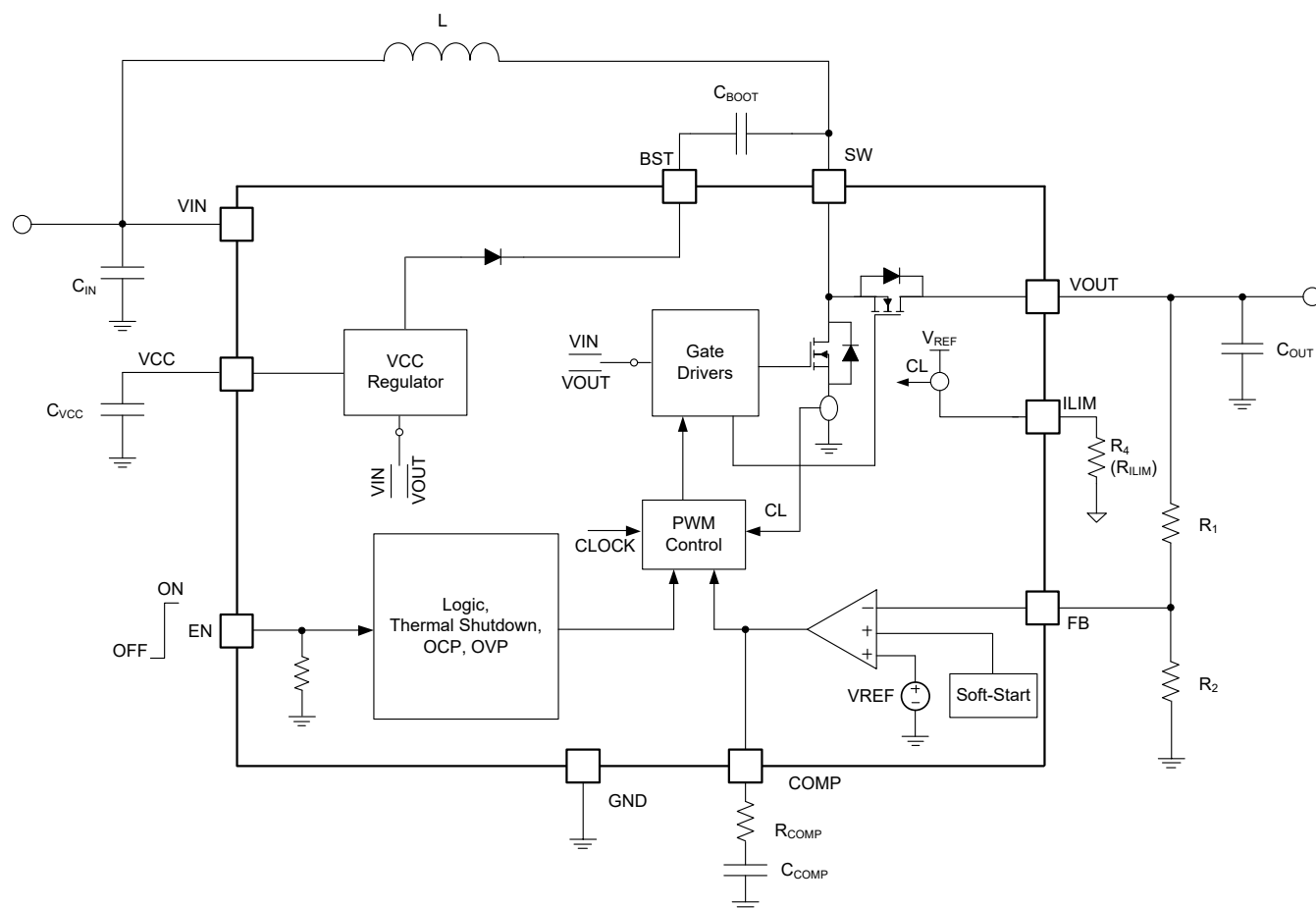
Figure 2. Block Diagram
