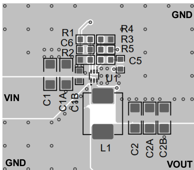
Figure 6. PCB Top Layer
