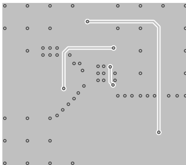
Figure 7. PCB Bottom Layer
