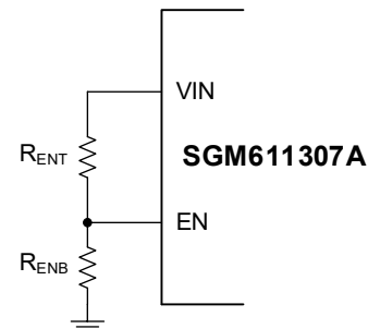
Figure 3. System UVLO by Enable Divider
