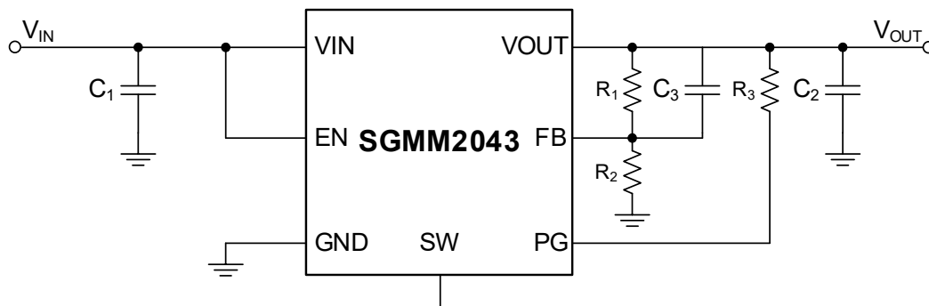
Figure 1. Simplified Schematic
