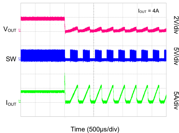
Short-Circuit, Entry (SGMM2043A)
