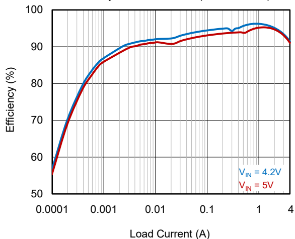
Efficiency vs. Load Current (SGMM2043A)
