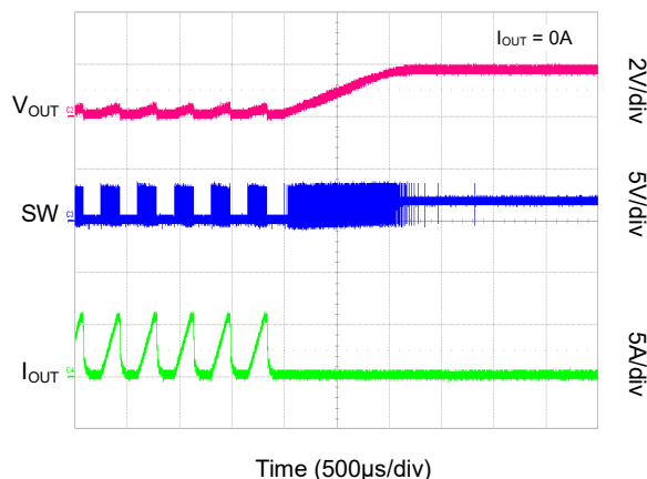
Short-Circuit, Recovery (SGMM2043A)
