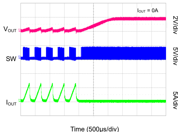
Short-Circuit, Recovery (SGMM2043B)
