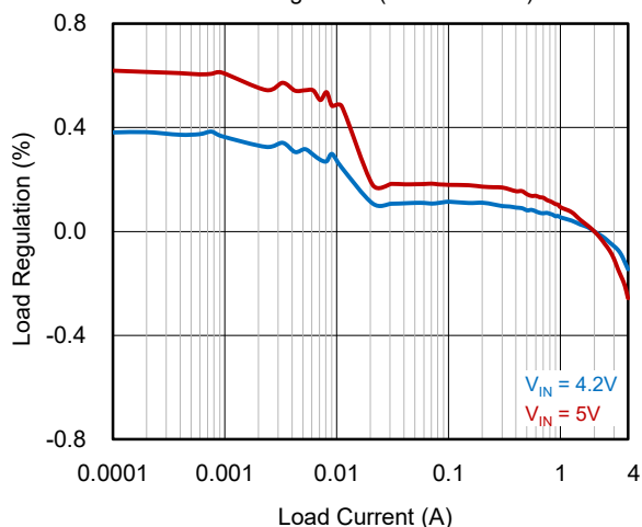
Load Regulation (SGMM2043A)
