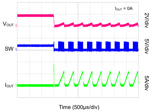
Short-Circuit, Entry (SGMM2043A)
