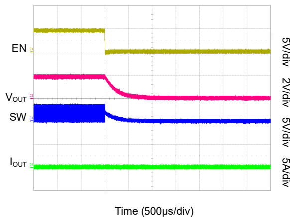
Shutdown without Load (SGMM2043B)
