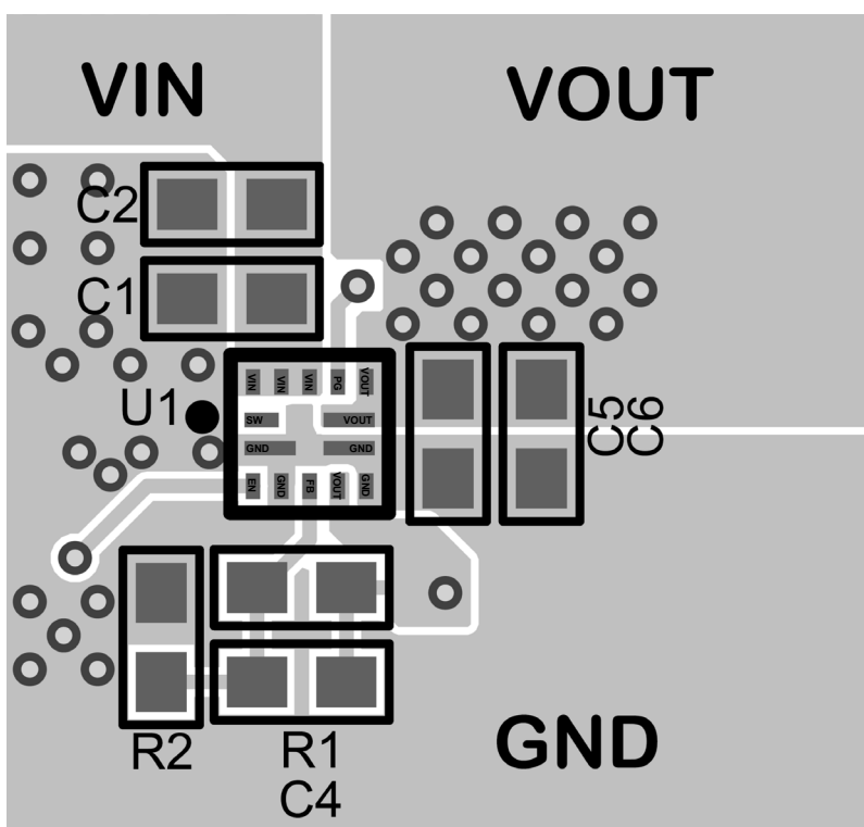
Figure 4. PCB Example-Top Layer
