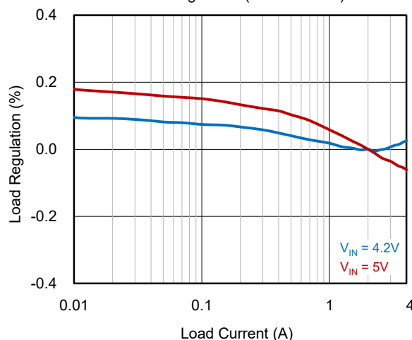
Load Regulation (SGMM2043B)
