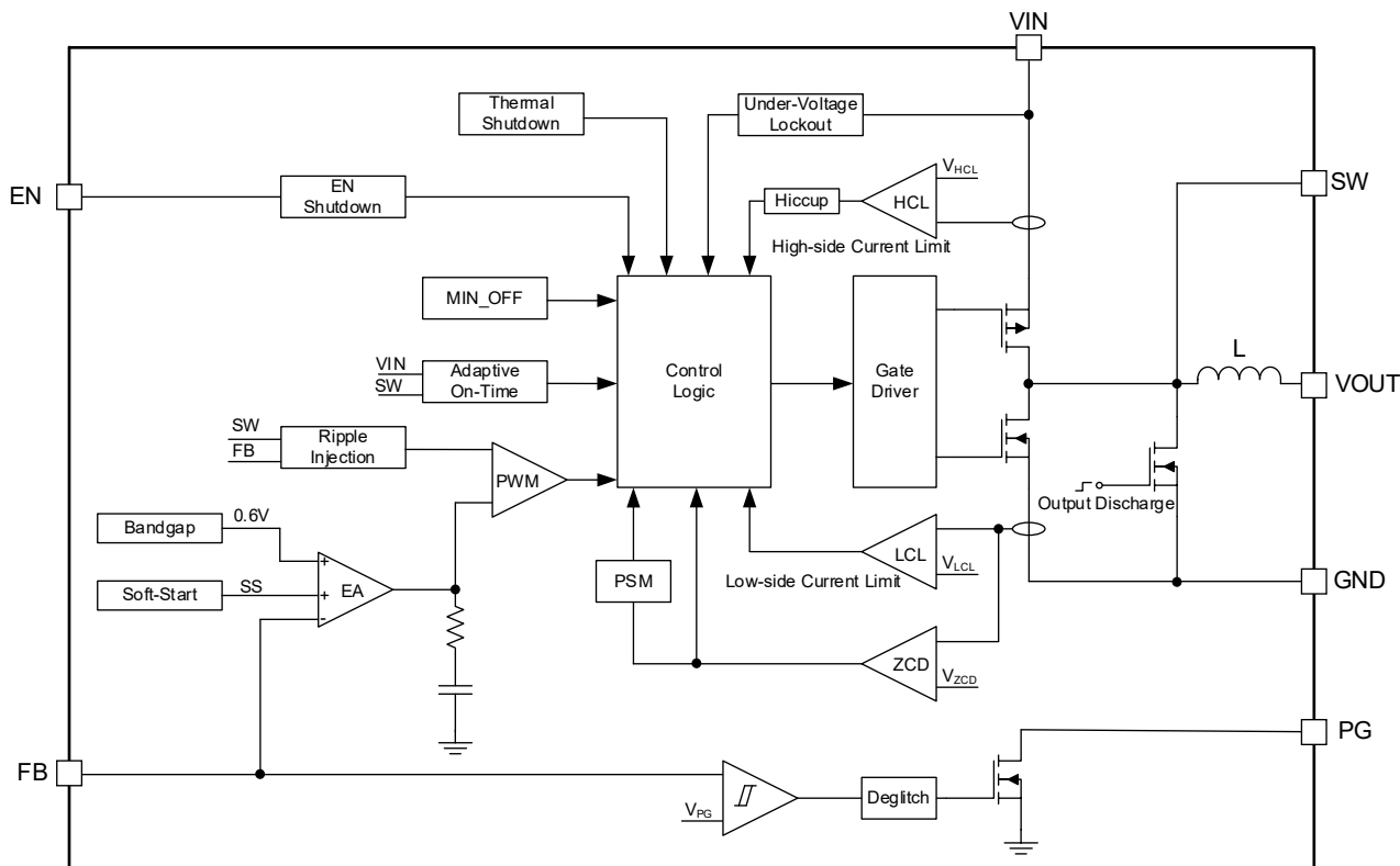
Figure 2. Block Diagram
