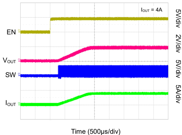
Startup with Load (SGMM2043A)
