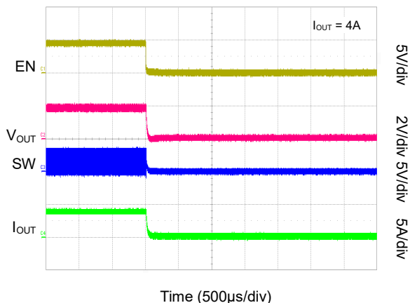
Shutdown with Load (SGMM2043A)
