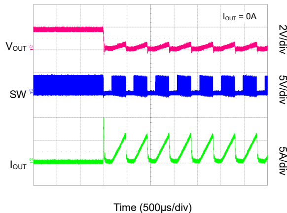
Short-Circuit, Entry (SGMM2043B)
