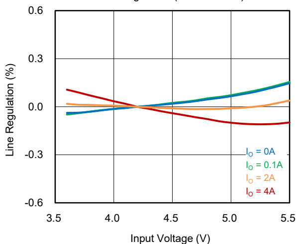
Line Regulation (SGMM2043B)
