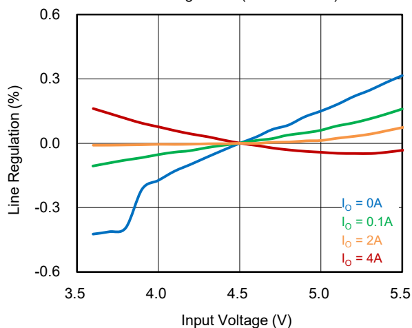
Line Regulation (SGMM2043A)
