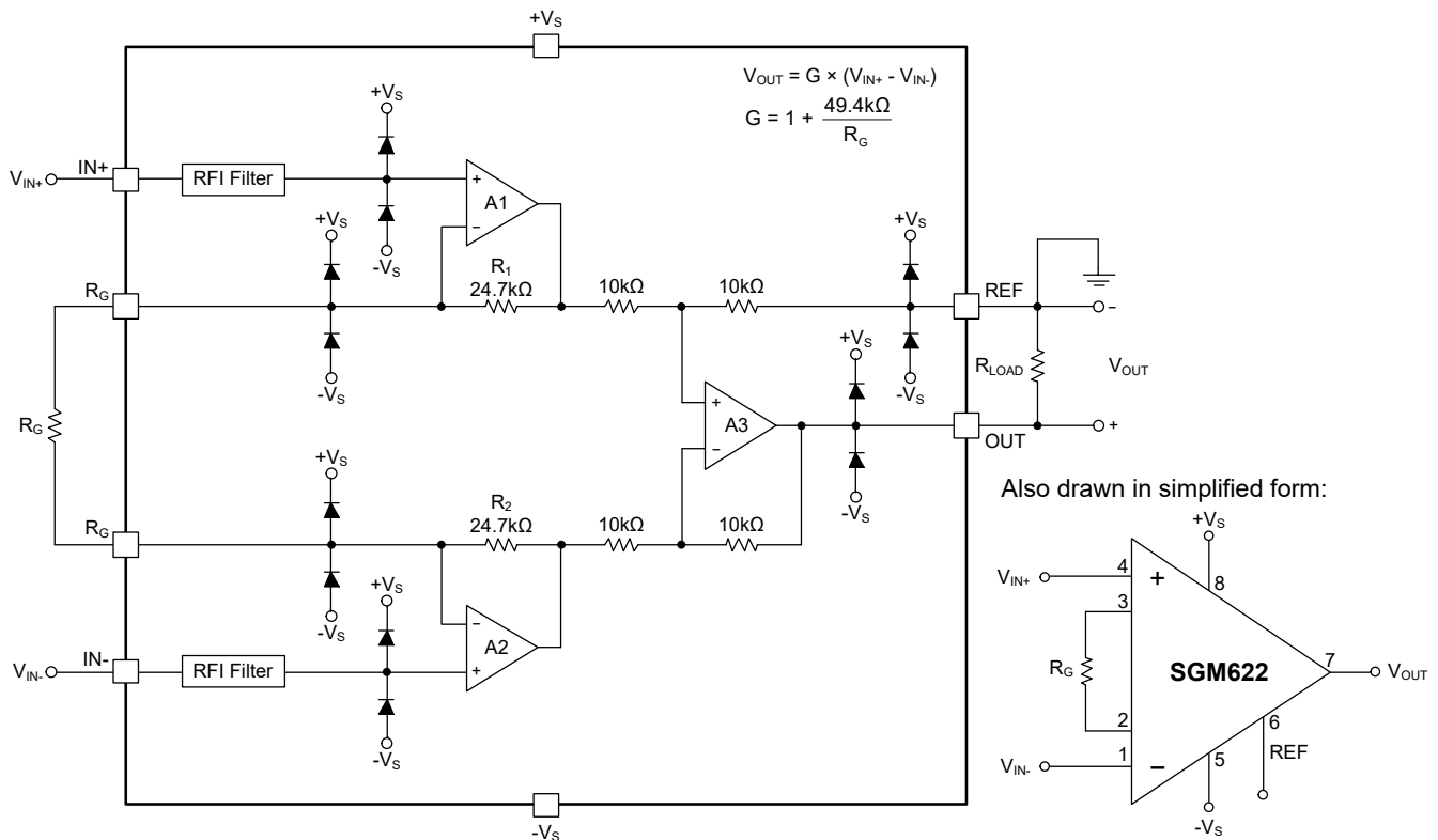
Figure 1. Simplified Schematic
