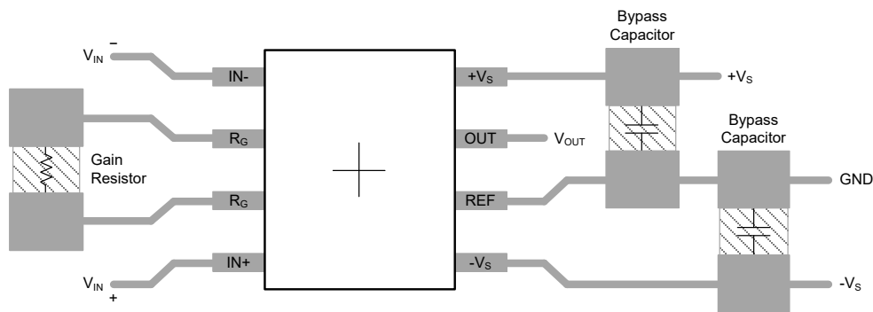
Figure 13. PCB Layout Example
