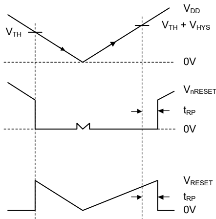
Figure 2. Timing Diagram
