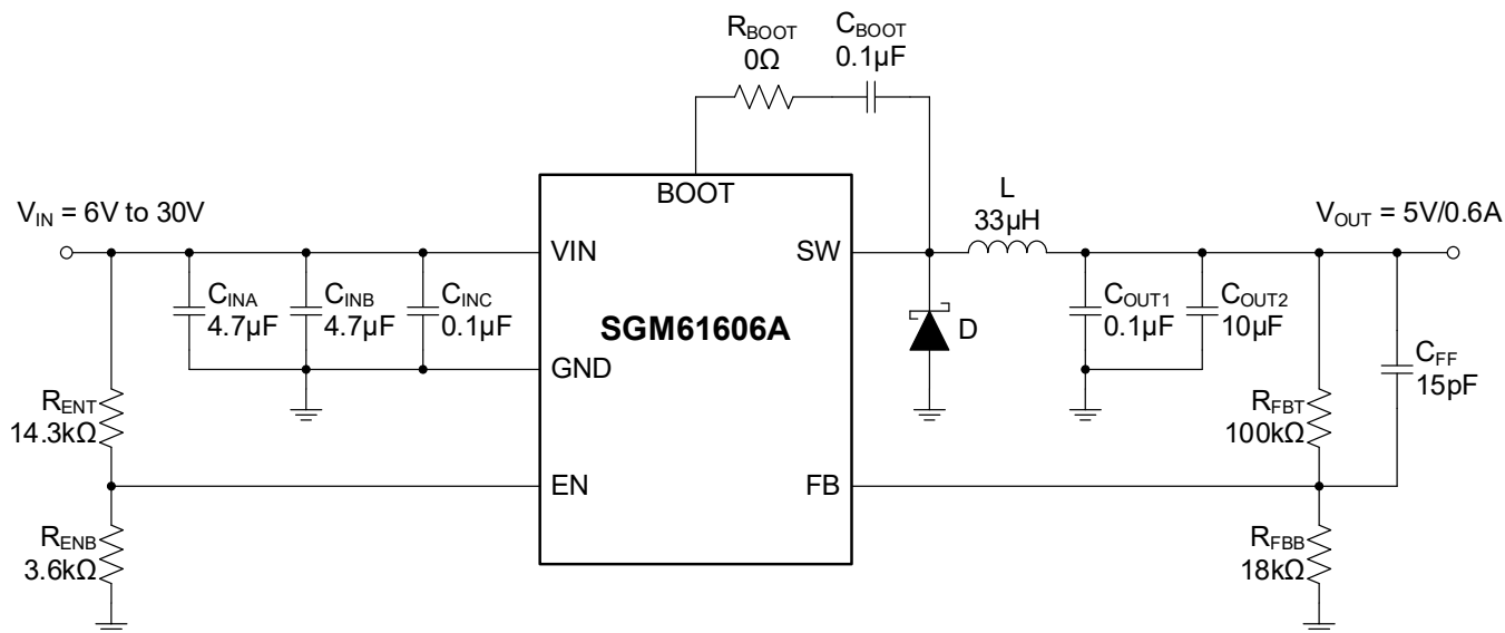
Figure 6. A Reference Design for 5V/0.6A Application
