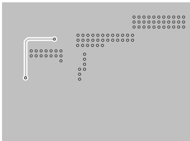
Figure 8. PCB Bottom Layer
