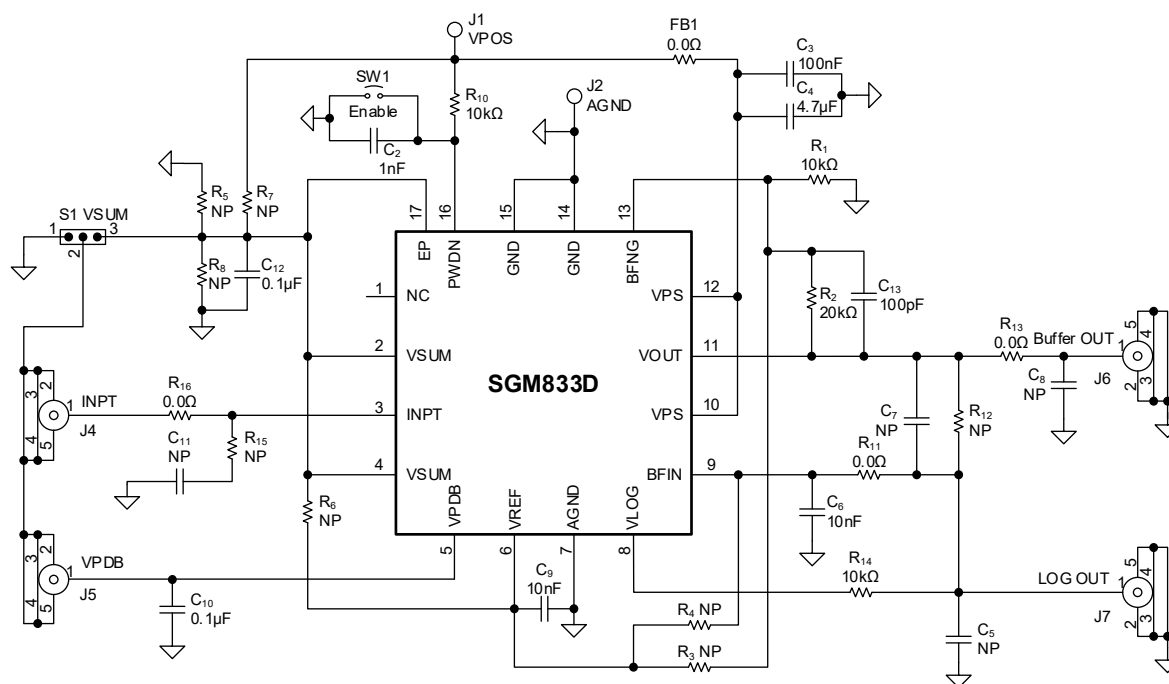
Figure 12. SGM833D Evaluation Board Schematic
