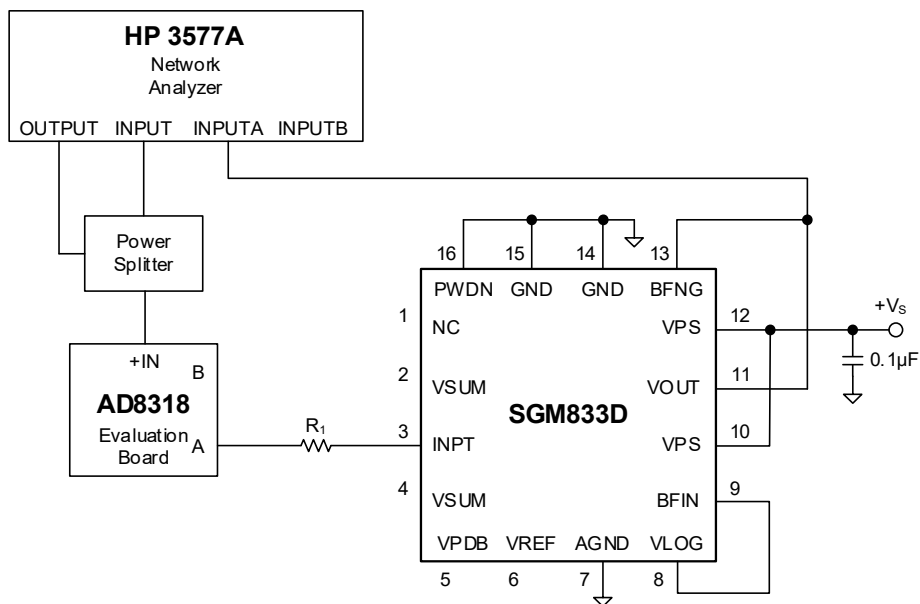
Figure 5. Converter Small Signal Bandwidth Measurement Setup
