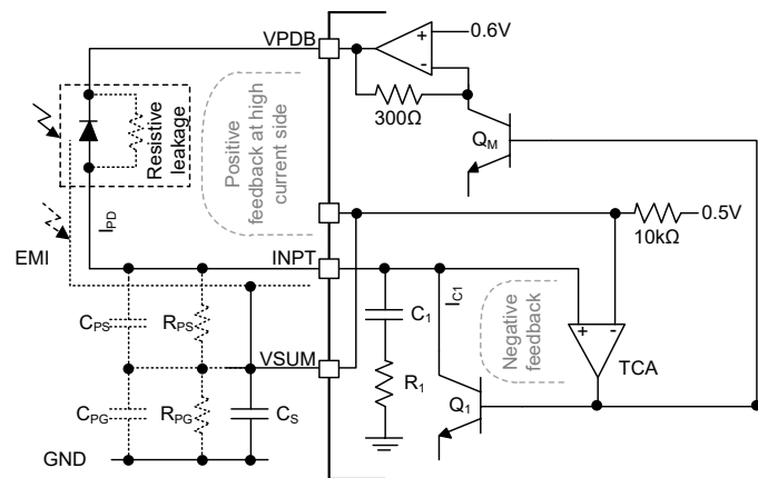
Figure 8. Conversion Loop and Active Shielding Loop
