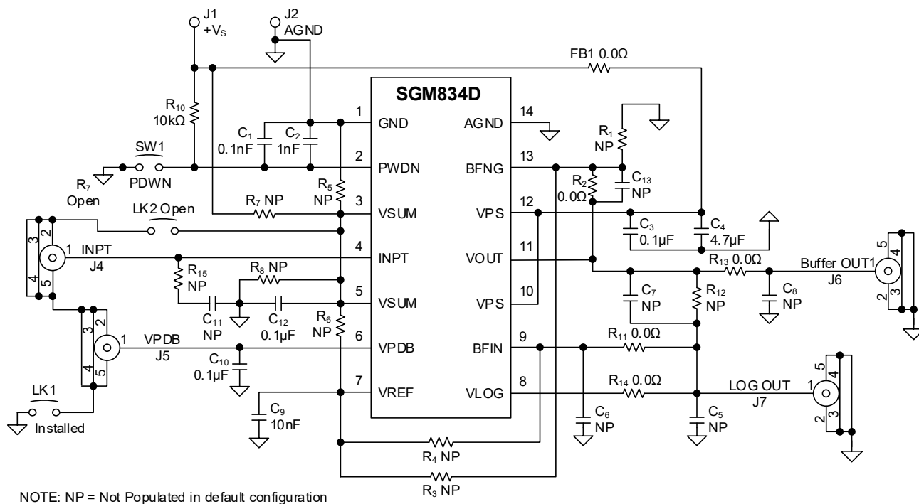
Figure 12. SGM834D Evaluation Board Schematic
