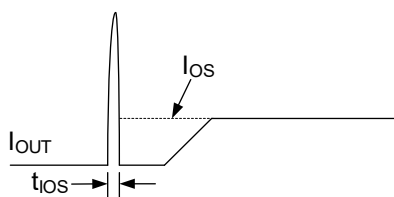
Figure 6. Output Short-Circuit Parameters
