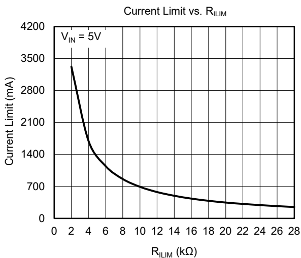
Figure 7. Current Limit Threshold ( I_{LIM} ) vs. Current Limit Programming Resistor ( R_{ILIM} )
