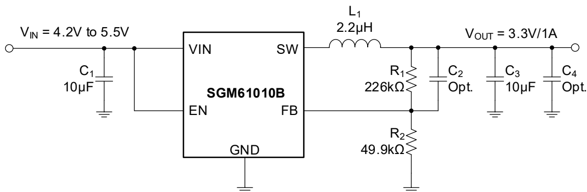
Figure 8. 3.3V Output Voltage Application
