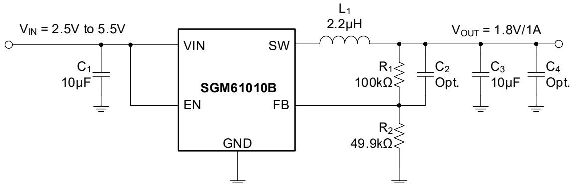
Figure 3. SGM61010B Application Example with 1.8V/1.0A Output
