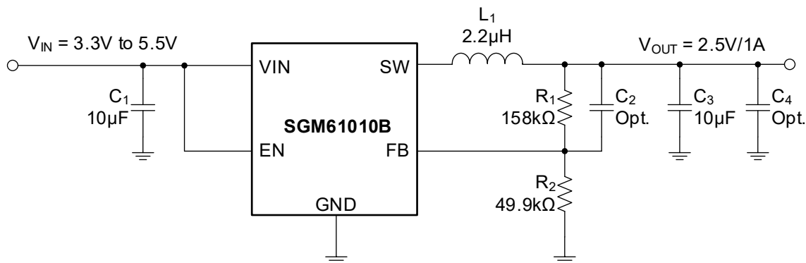
Figure 7. 2.5V Output Voltage Application
