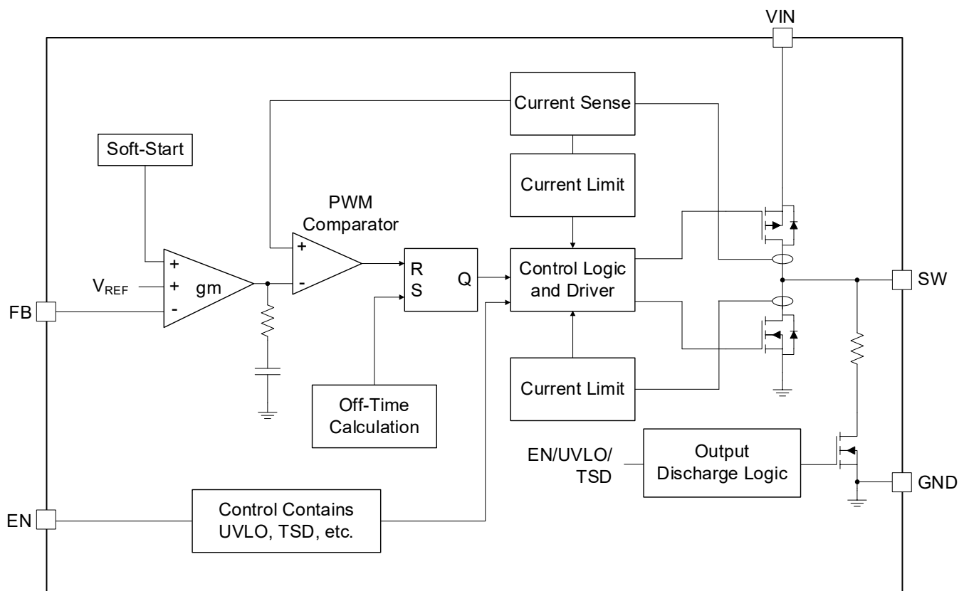
Figure 2. Block Diagram
