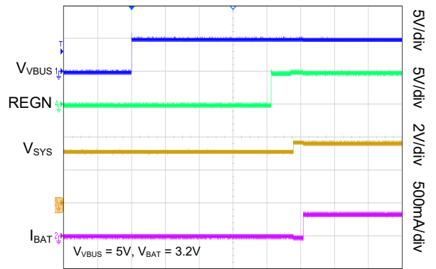
Time (50ms/div)
