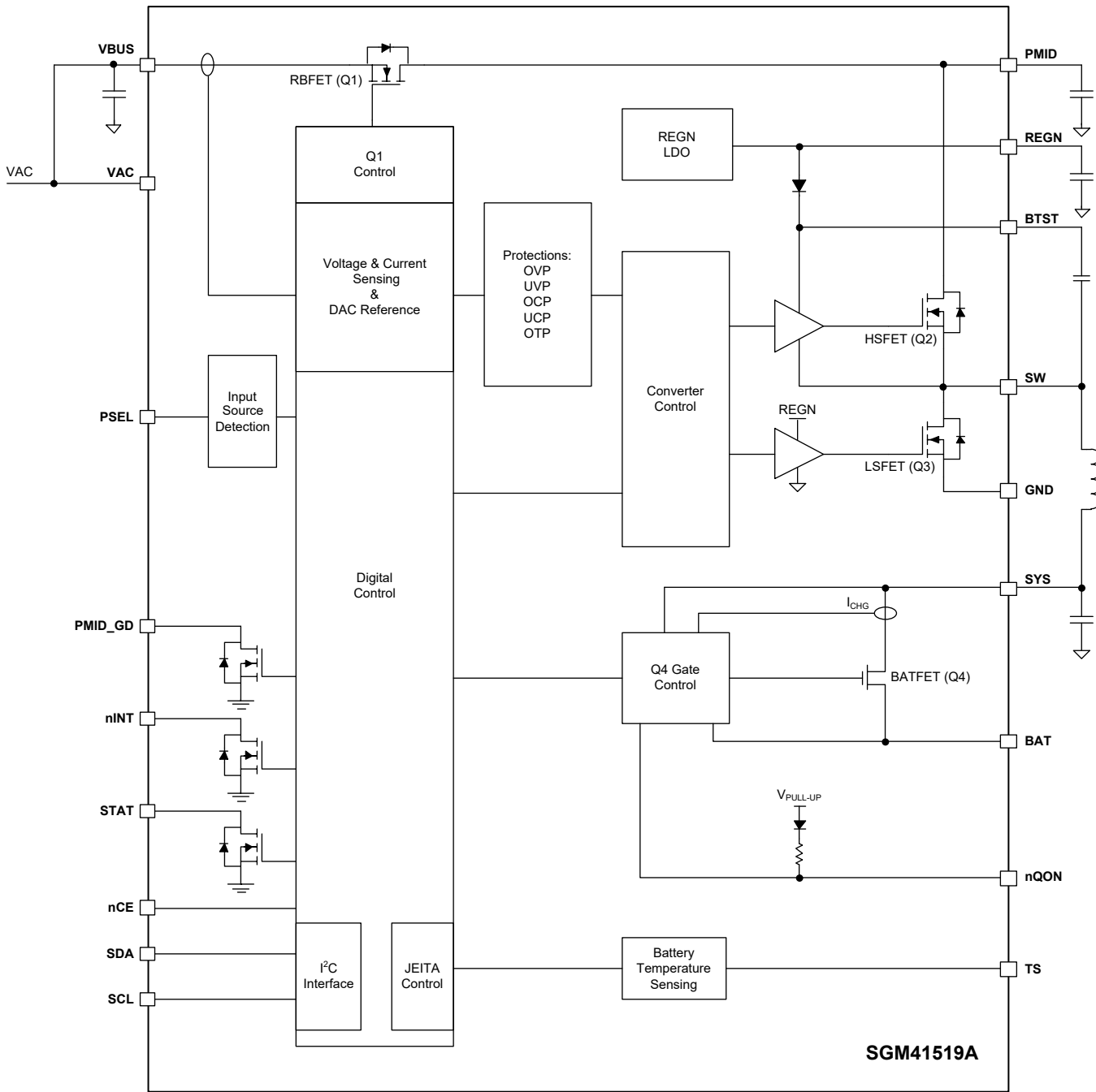
Figure 2. Block Diagram
