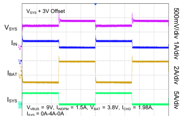
Time (2ms/div)
