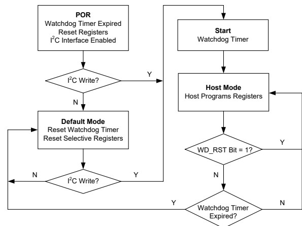
Figure 3. Watchdog Timer Flow Chart
