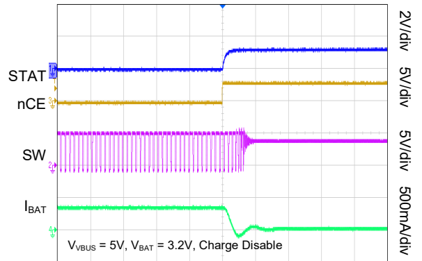
Time (5µs/div)
