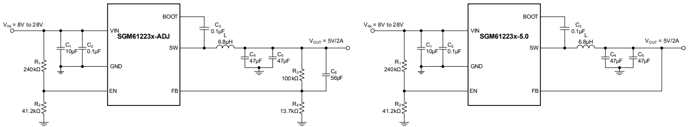
Figure 6. A Reference Design for 5V/2A Application
