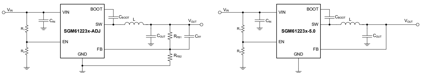
Figure 1. Typical Application Circuit
