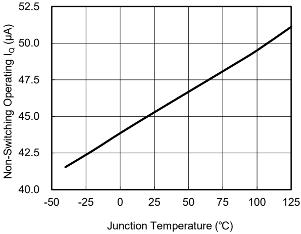
Non-Switching Operating I_Q vs. Junction Temperature (SGM61223A)
