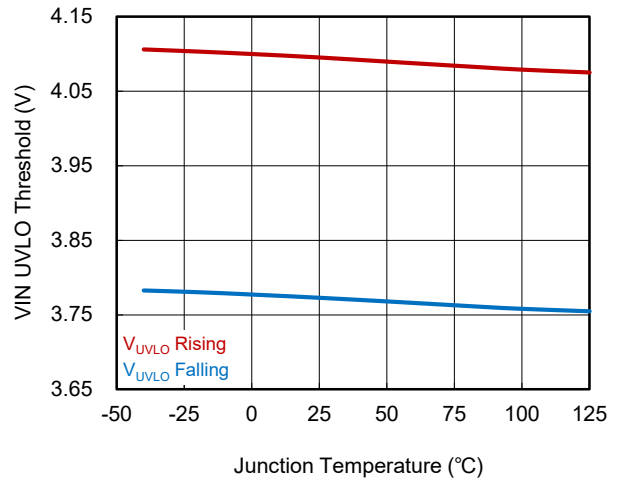
VIN UVLO Threshold vs. Junction Temperature
