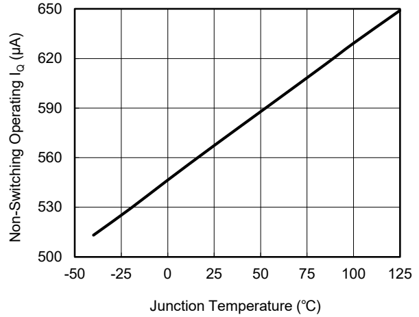
Non-Switching Operating I_Q vs. Junction Temperature (SGM61223B)
