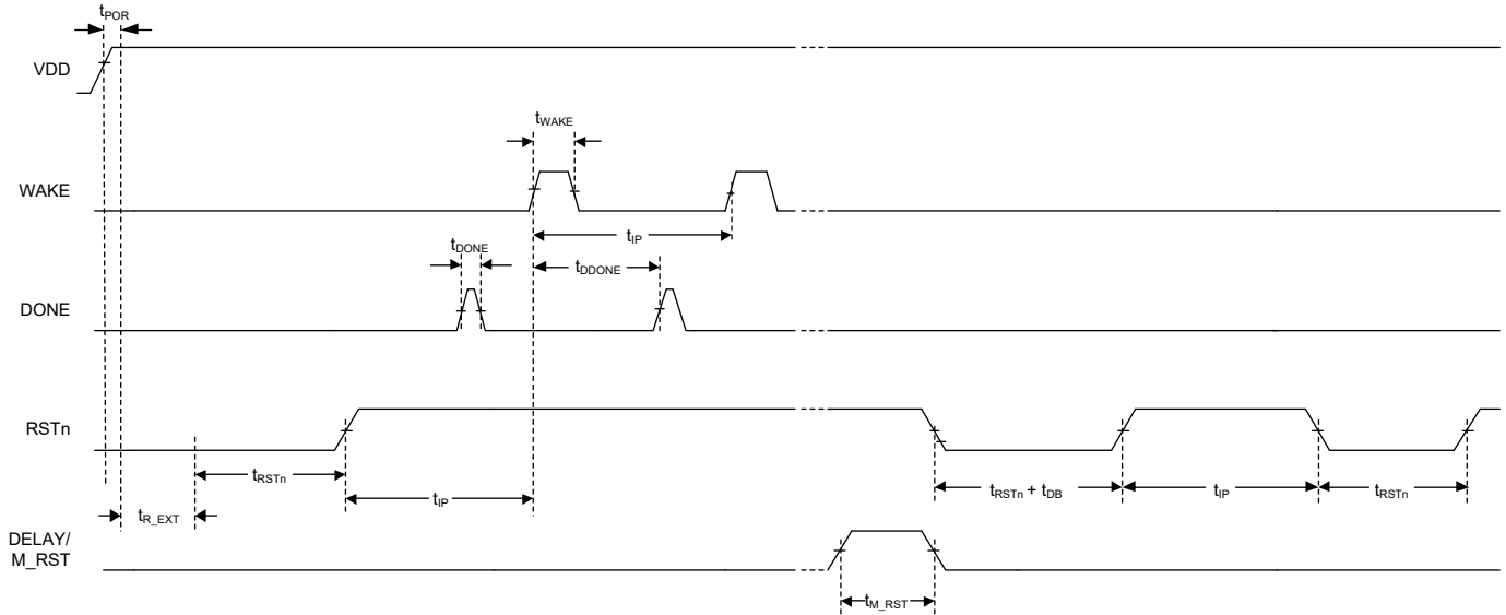
Figure 2. Timing Diagram
