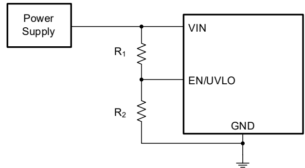
Figure 4. Adjustable Supply UVLO Threshold
