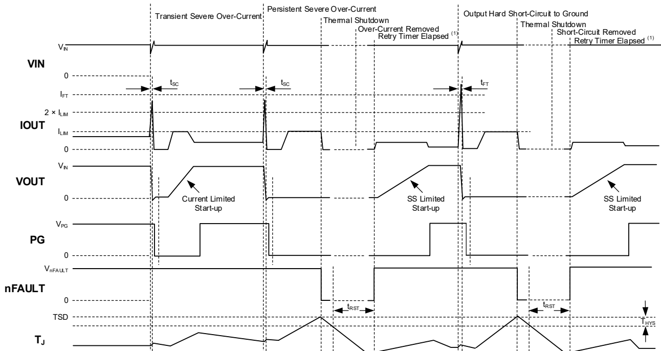
Figure 8. Short-Circuit Response
