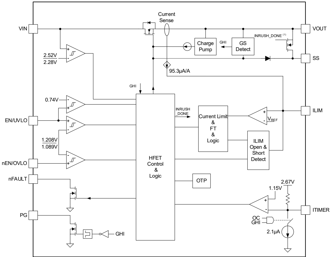
Figure 3. Block Diagram
