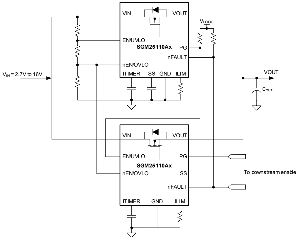
Figure 13. Two SGM25110Ax Devices Connected in Parallel for Higher Steady-State Current Capability
