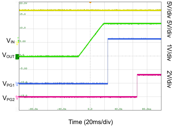
Parallel Devices Sequencing during Startup
