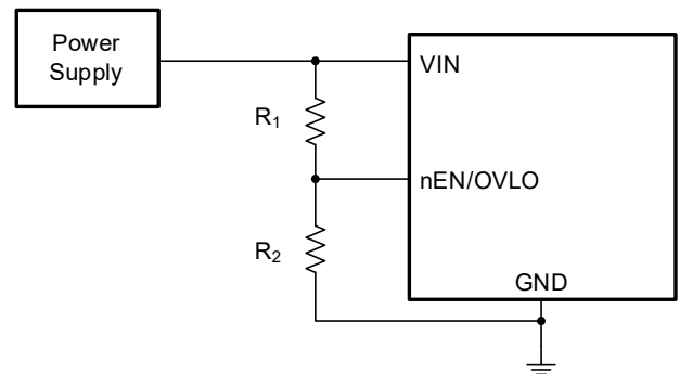
Figure 5. Adjustable Over-Voltage Protection
