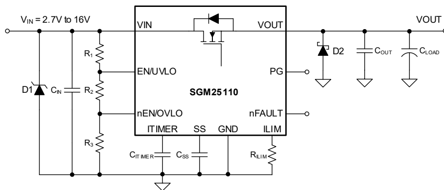
Figure 17. Circuit Implementation with Optional Protection Components
