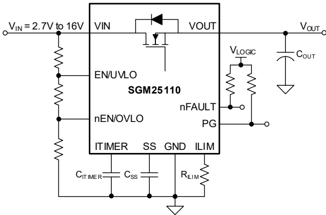
Figure 12. Single Device, Self-Controlled
