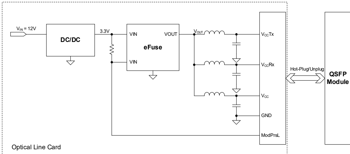
Figure 14. Power Tree Block Diagram of a Typical Optical Line Card
