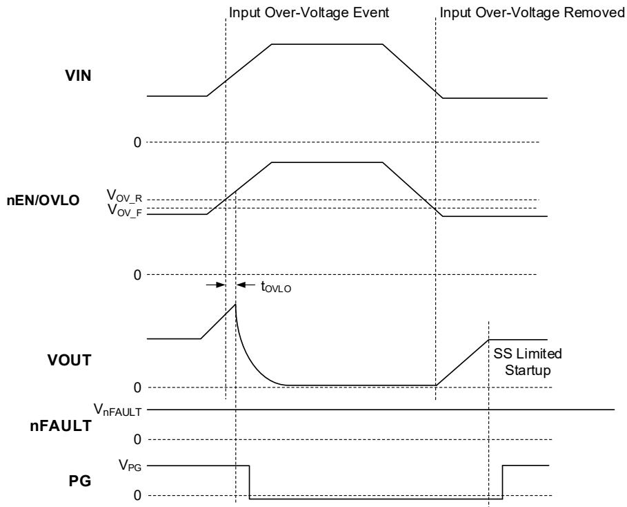
Figure 6. SGM25110Ax Over-Voltage Lockout and Recovery
