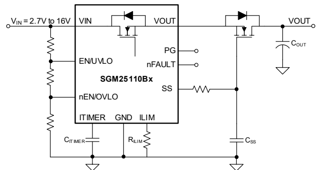
Figure 11. Reverse Current Blocking Using External FET-SGM25110Bx
