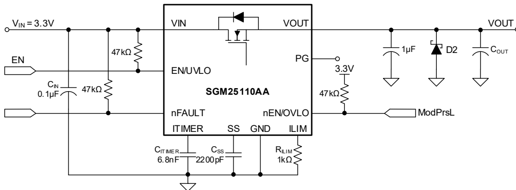
Figure 15. Optical Module Port Protection
