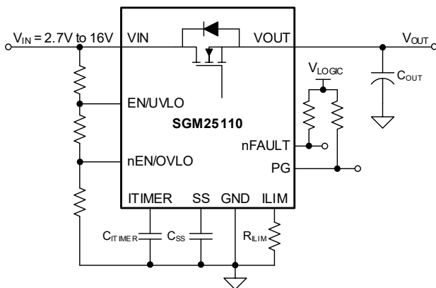
Figure 1. Simplified Schematic
