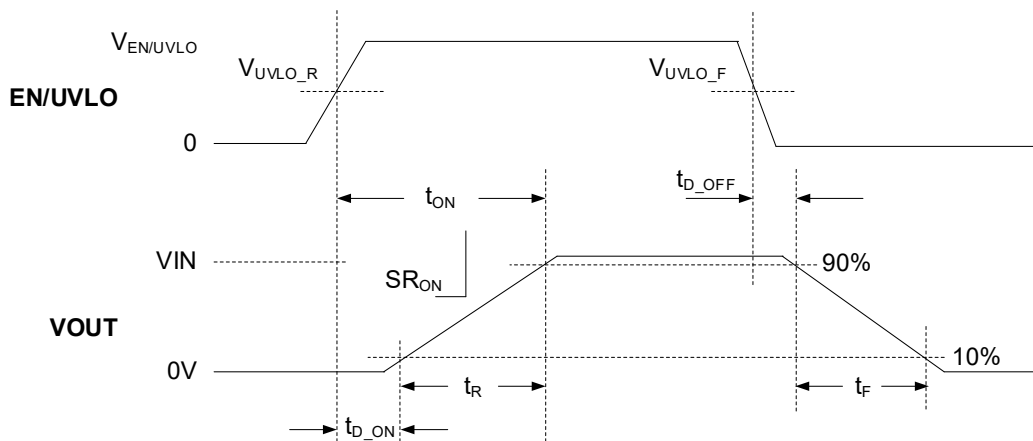
Figure 2. Switching Times
