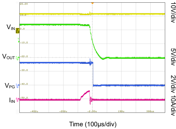
Over-Voltage Shutdown
