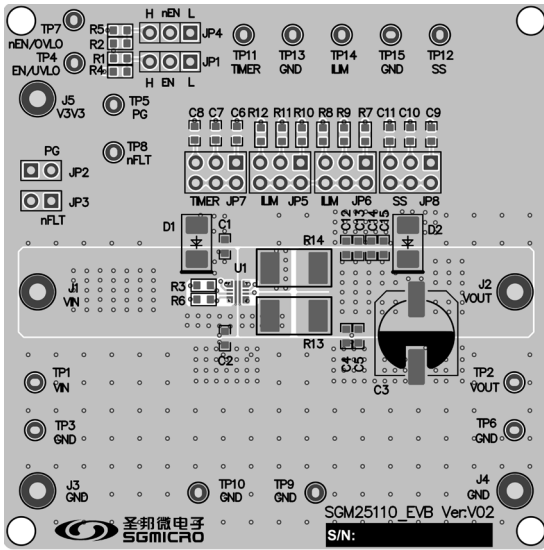
Figure 18. PCB Top Layer
