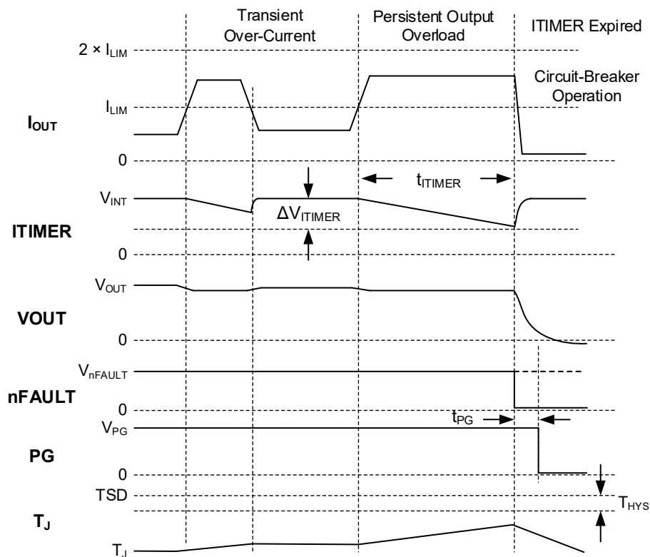
Figure 7. SGM25110Ax Over-Current Response
