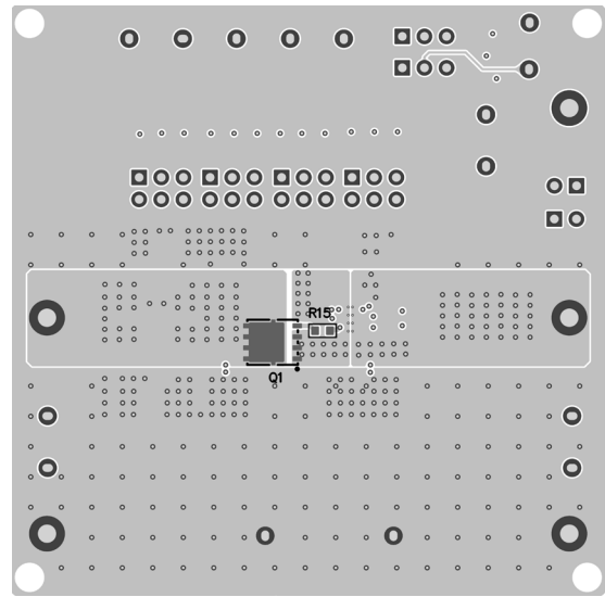
Figure 19. PCB Bottom Layer
