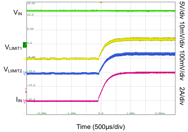
Parallel Devices Load Current During Steady-State
