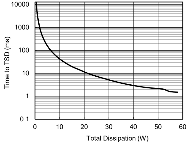
Figure 16. Thermal Shutdown Plot during Inrush
