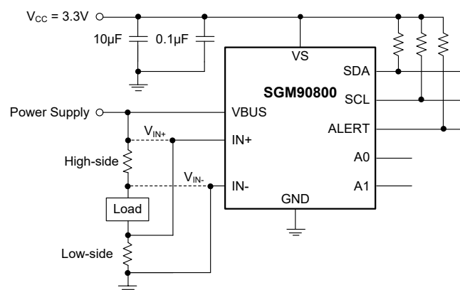
Figure 1. High-side/Low-side Sensing Application Circuit
