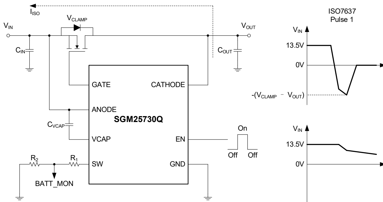
Figure 6. SGM25730Q Operation during V_{DS} Clamp Mode
