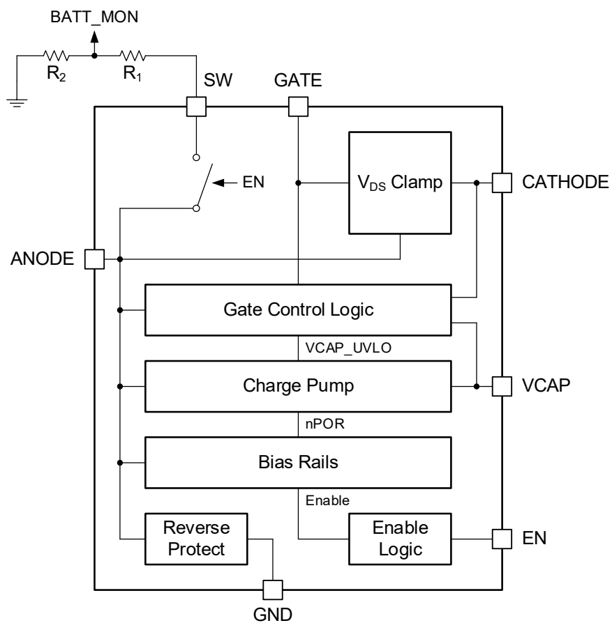
Figure 3. Block Diagram
