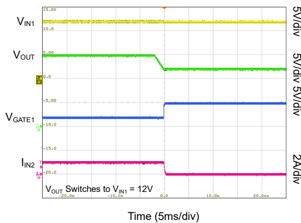
ORing - V_{\text{IN}2} to V_{\text{IN}1} Switch Over
