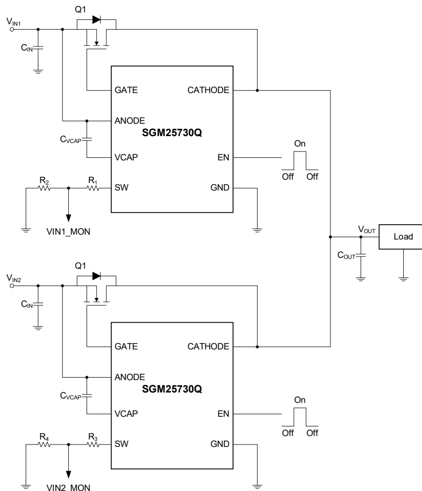
Figure 10. Typical ORing Application
