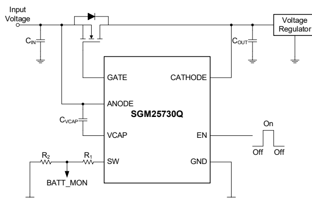
Figure 1. Simplified Schematics
