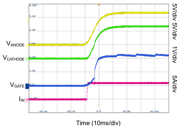
Start-Up with 6A Load
