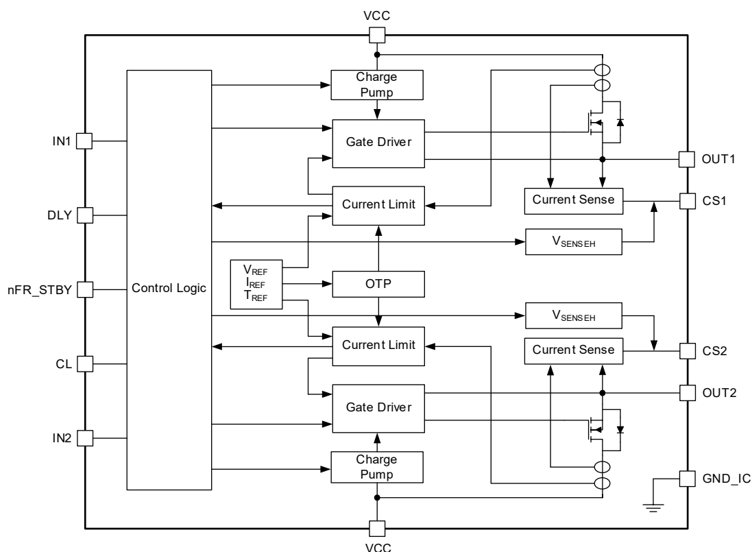
Figure 2. Block Diagram
