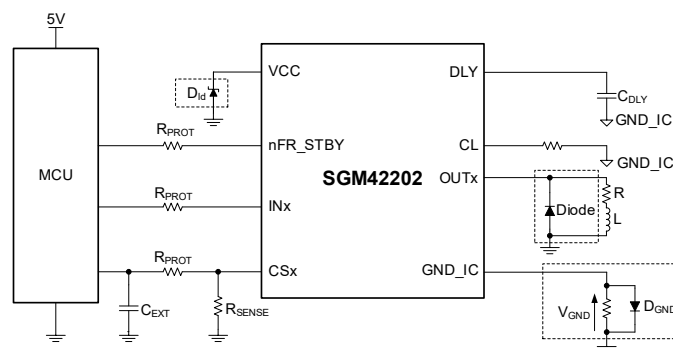
Figure 1. Typical Schematic
