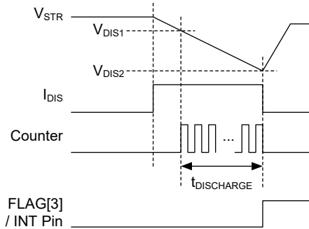
Figure 7. Measuring Capacitance with 500Hz Counter
