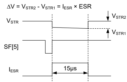
Figure 6. ESR Measurement Process
