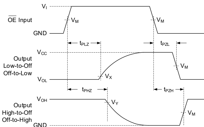
Figure 3. Latch Enable Input LE to Output Qn Propagation Delays, Pulse Width and Transition Times
