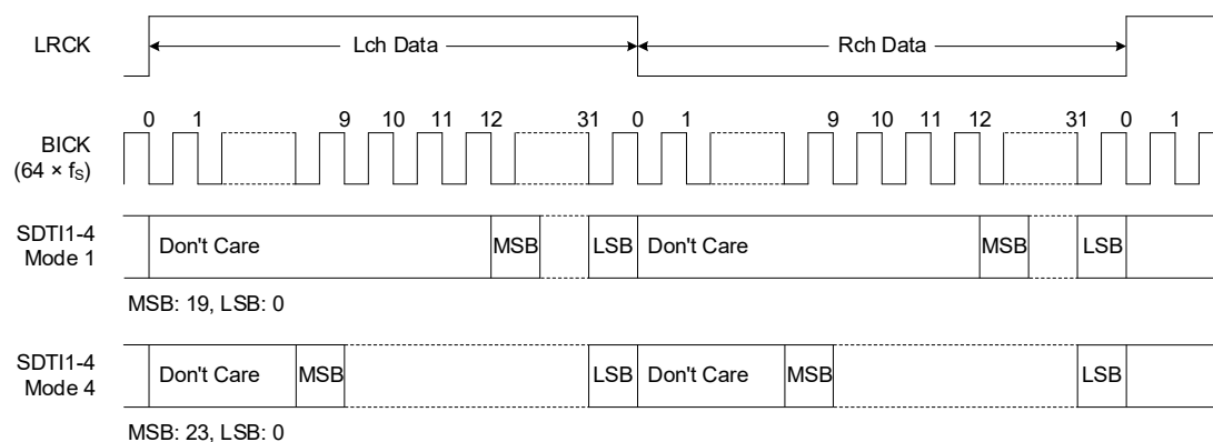
Figure 12. Audio Data Format Timing (Mode 1 and 4)
