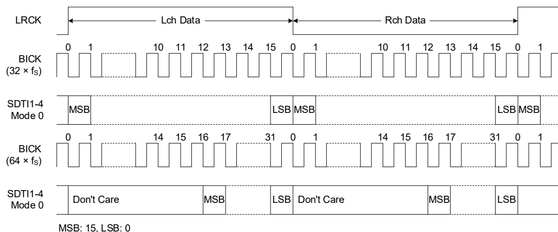
Figure 11. Audio Data Format Timing (Mode 0)
