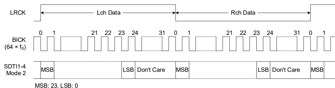
Figure 13. Audio Data Format Timing (Mode 2)
