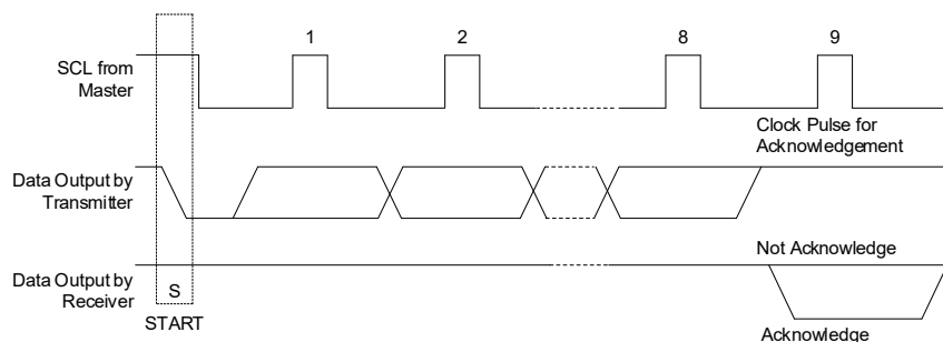
Figure 44. Acknowledge on the I²C-Bus Mode
