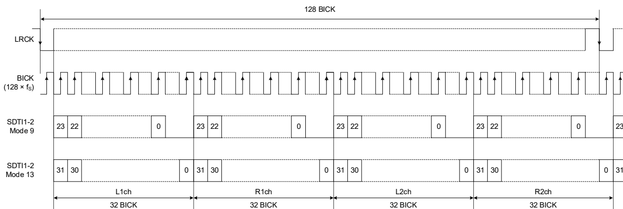
Figure 18. Audio Data Format Timing (Mode 9 and 13)
