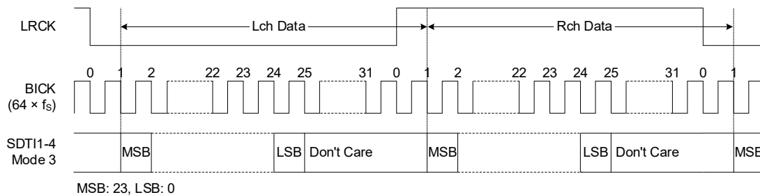
Figure 14. Audio Data Format Timing (Mode 3)
