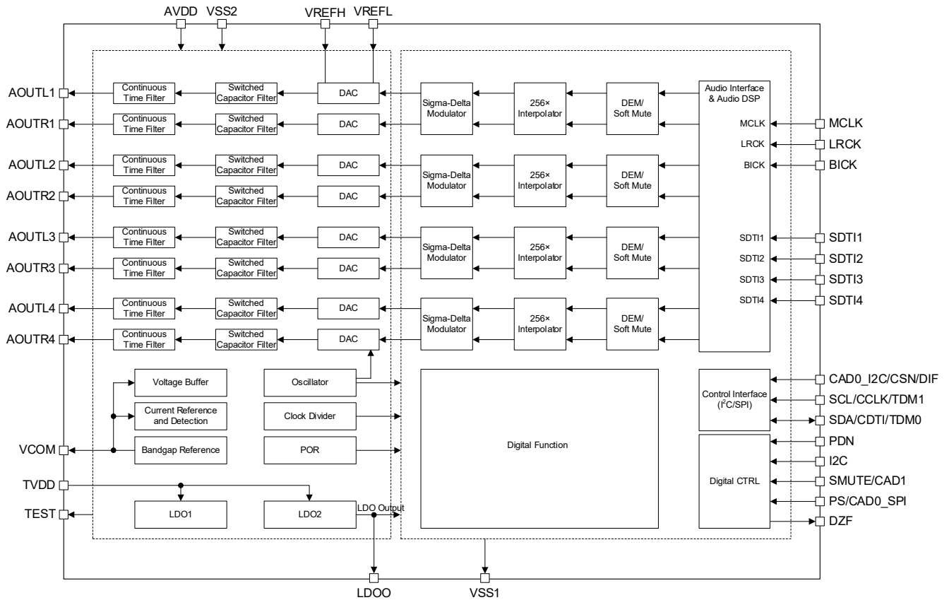
Figure 10. Block Diagram
