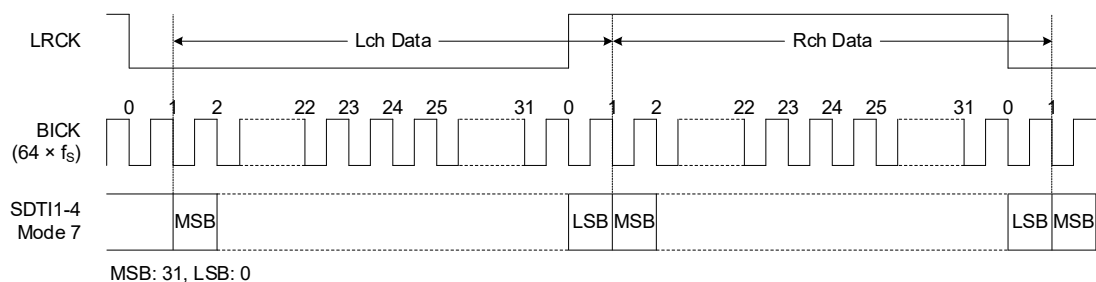
Figure 16. Audio Data Format Timing (Mode 7)
