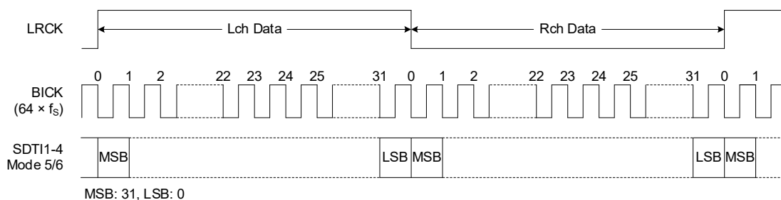
Figure 15. Audio Data Format Timing (Mode 5 and 6)
