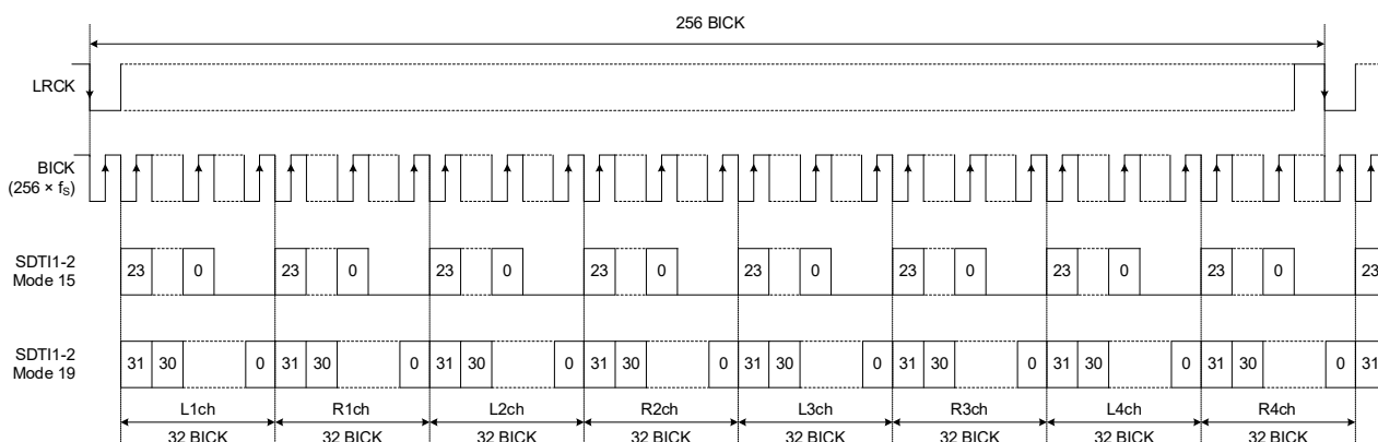
Figure 21. Audio Data Format Timing (Mode 15 and 19)
