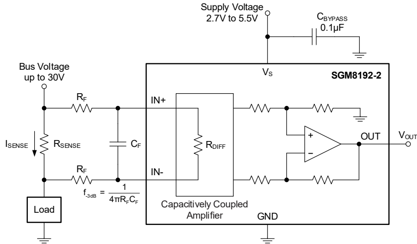
Figure 7. Filtering at Input
