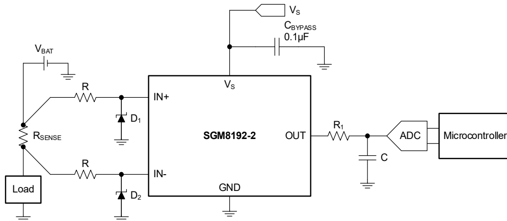
Figure 6. Typical Application Circuit for Battery-Powered System
