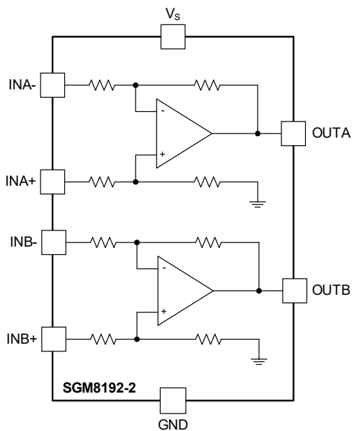
Figure 2. Block Diagram
