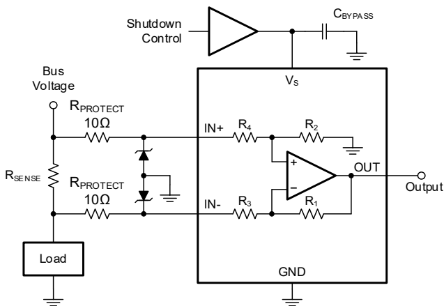
Figure 8. Using Dual Diodes for Absorbing Supply Transient
