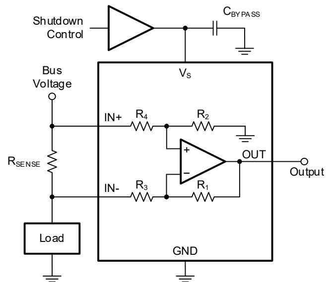
Figure 5. Shutting Down the Current Shunt Monitor
