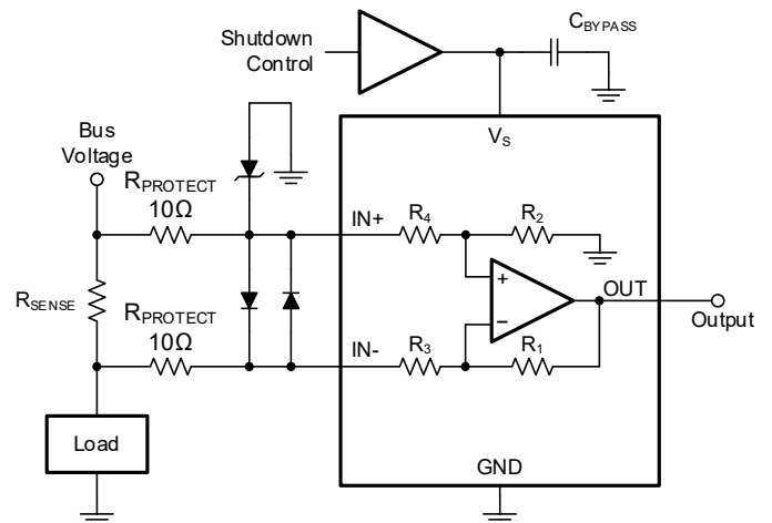
Figure 9. Using Transzorb and Input Clamps for Absorbing Supply Transient
