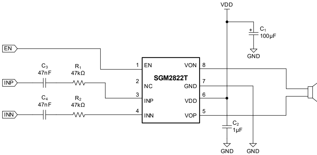
Figure 6. Differential Audio Input (for Mobile Phone Application)
