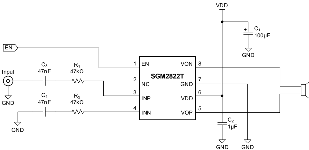
Figure 7. Single-Ended Audio Input Application
