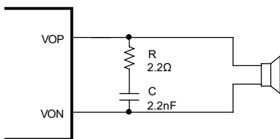
Figure 5. RC Snubber Circuit
