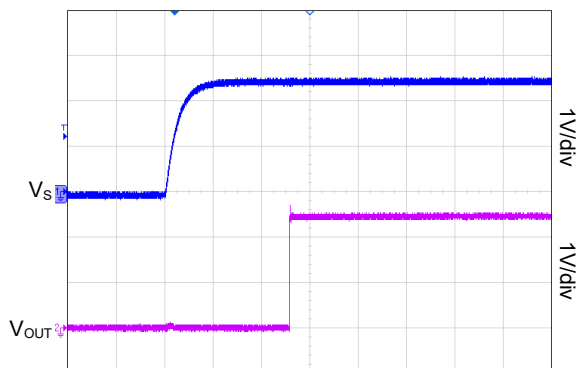
Power-Up Delay (OUT)
