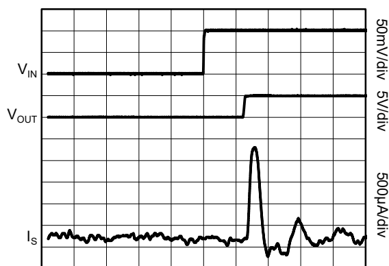
Switching Current (OUT Rising Edge)
