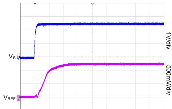
Power-Up Delay (REF)
