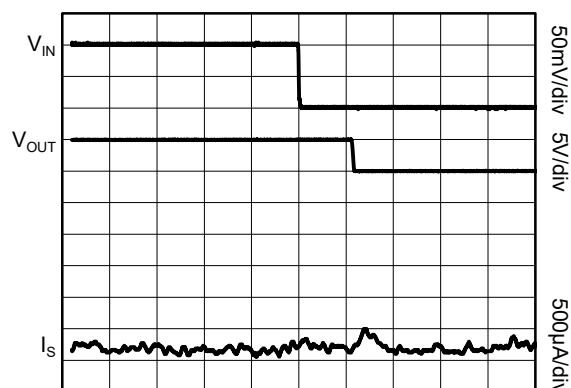
Switching Current (OUT Falling Edge)
