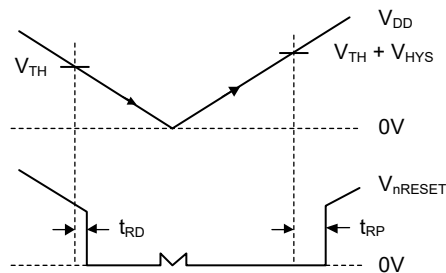
Figure 2. Timing Diagram
