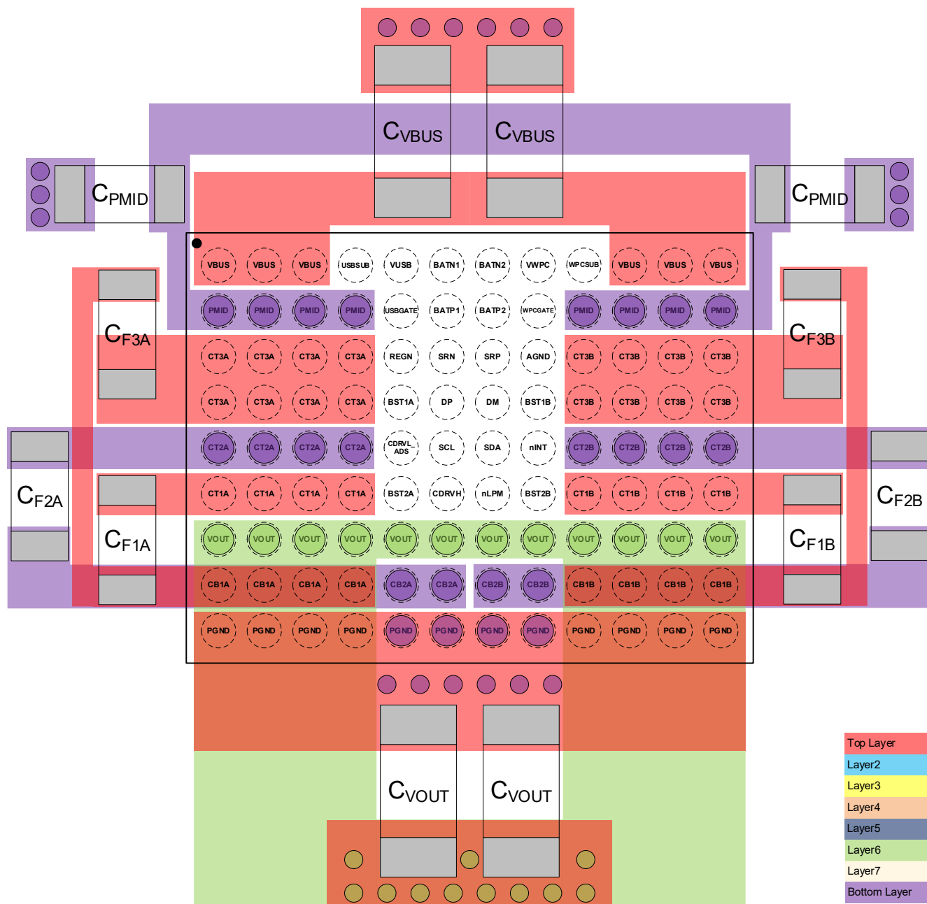
Figure 10. PCB Layout Reference
