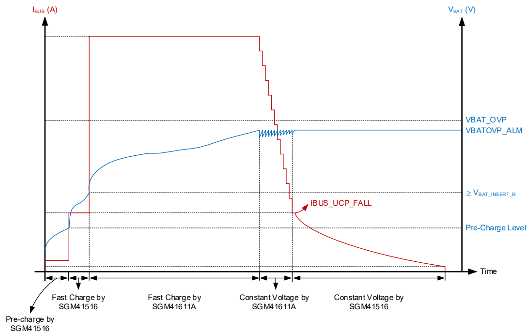
Figure 7. SGM41611A System Charging Profile
