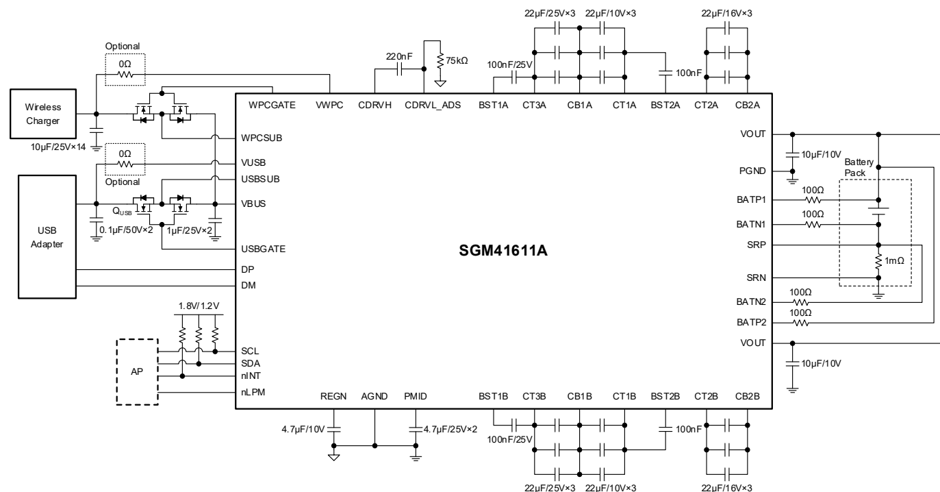
Figure 11. Typical Application Circuit of SGM41611A
