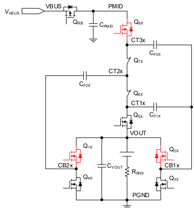
Figure 4. Power Stage of Single Channel 2:1/1:2 Switched-Capacitor Charger
