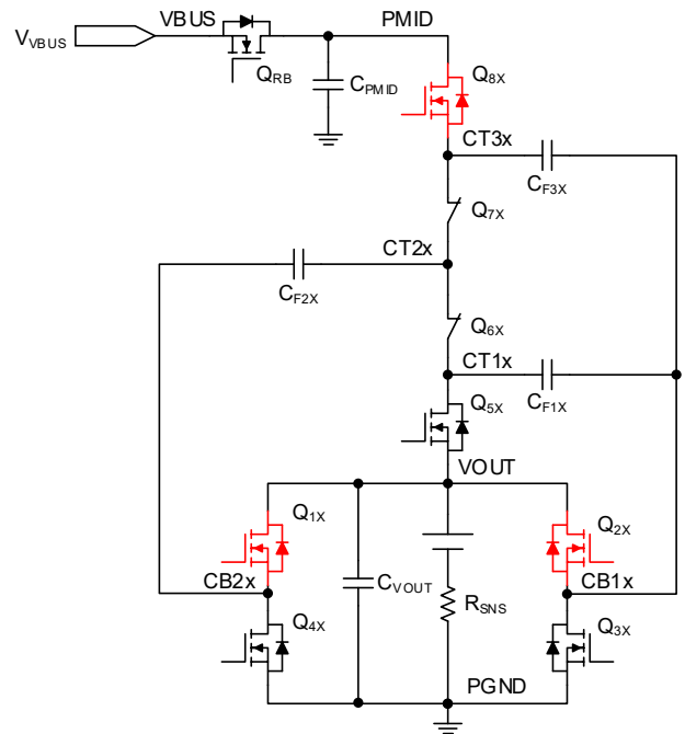
Figure 4. Power Stage of Single Channel 2:1/1:2 Switched-Capacitor Charger
