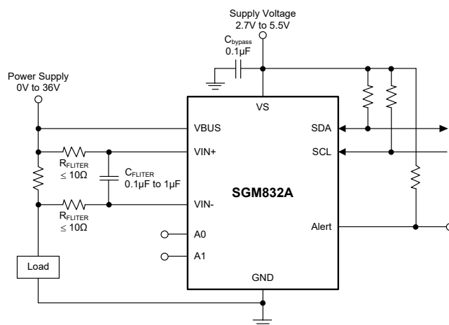
Figure 6. Input Filtering
