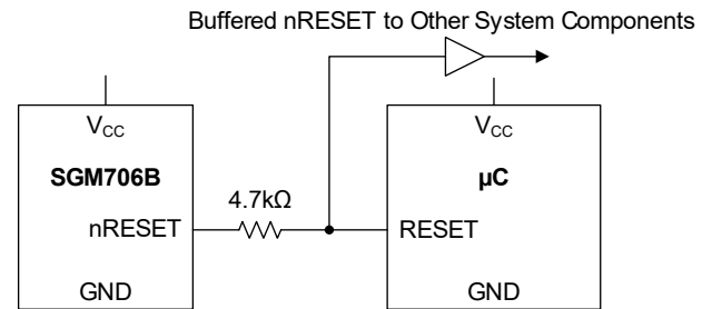
Figure 7. Interfacing to \mu\text{Cs} with Bidirectional Reset I/O
