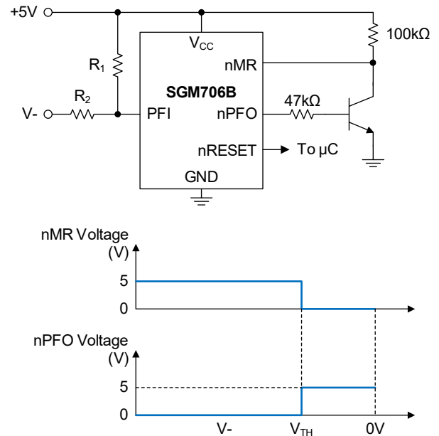
Figure 6. Negative Voltage Monitoring
