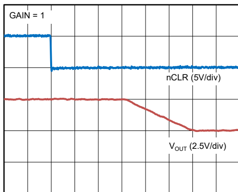
Clear to Zero-Scale (SGM71622R8ZC/SGM71622R8AZC)
