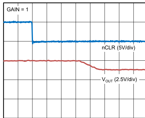
Clear to Mid-Scale (SGM71622R8MC/SGM71622R8AMC)
