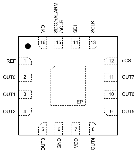
TQFN-3x3-16DL
