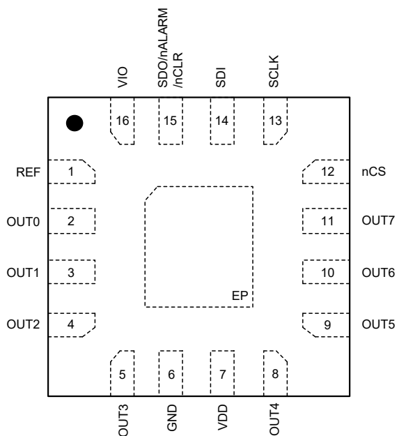
TQFN-3.5x3.5-16AL
