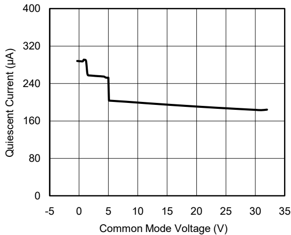
Quiescent Current vs. Common Mode Voltage
