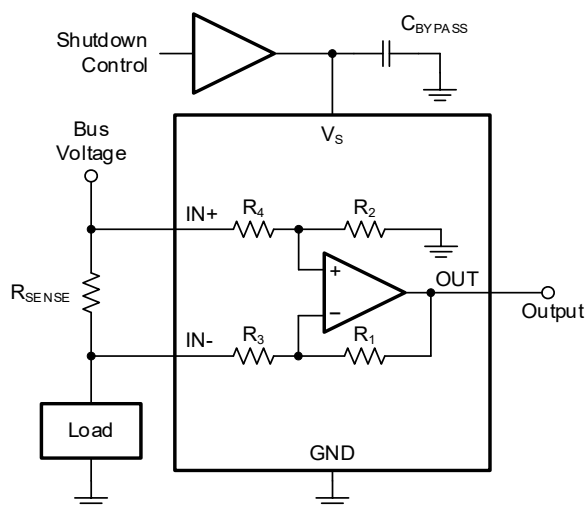
Figure 5. Shutting Down the Current Shunt Monitor
