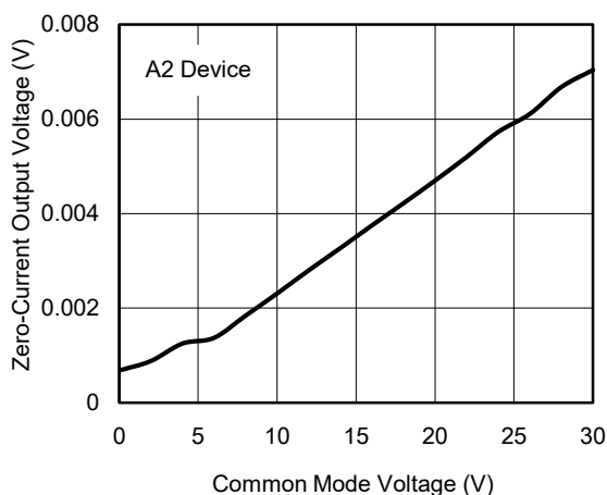
Figure 4. SGM8192-1xA2 Zero-Current Output Voltage vs. Common Mode Voltage
