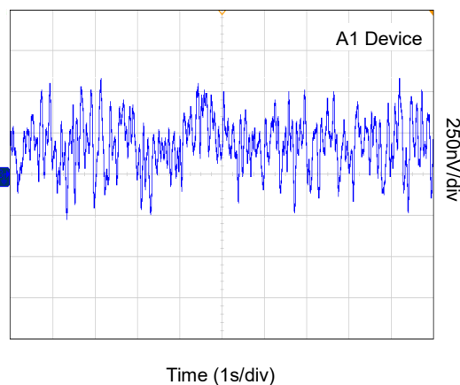
0.1Hz to 10Hz Voltage Noise (Referred-to-Input)
