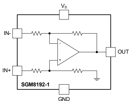
Figure 2. Block Diagram
