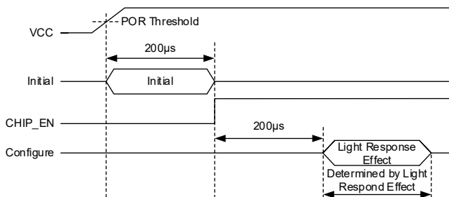
Figure 4. Power-up Timing
