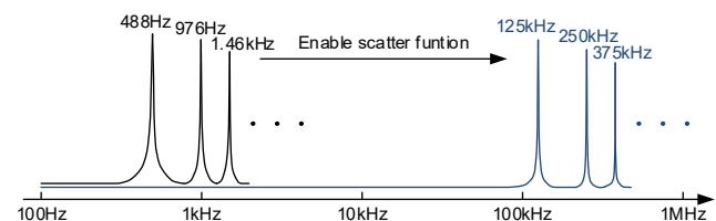
Figure 7. Output Frequency Spectrum
