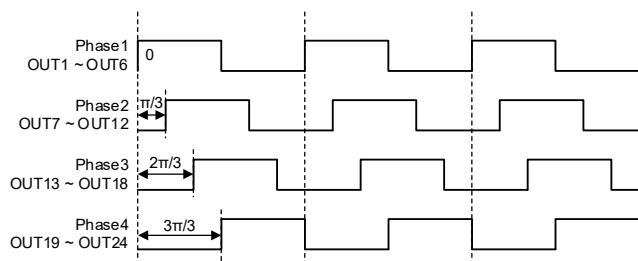
Figure 8. Phase Shift Scheme
