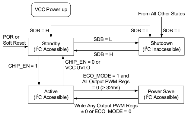
Figure 3. SGM31240 Operation State Diagram
