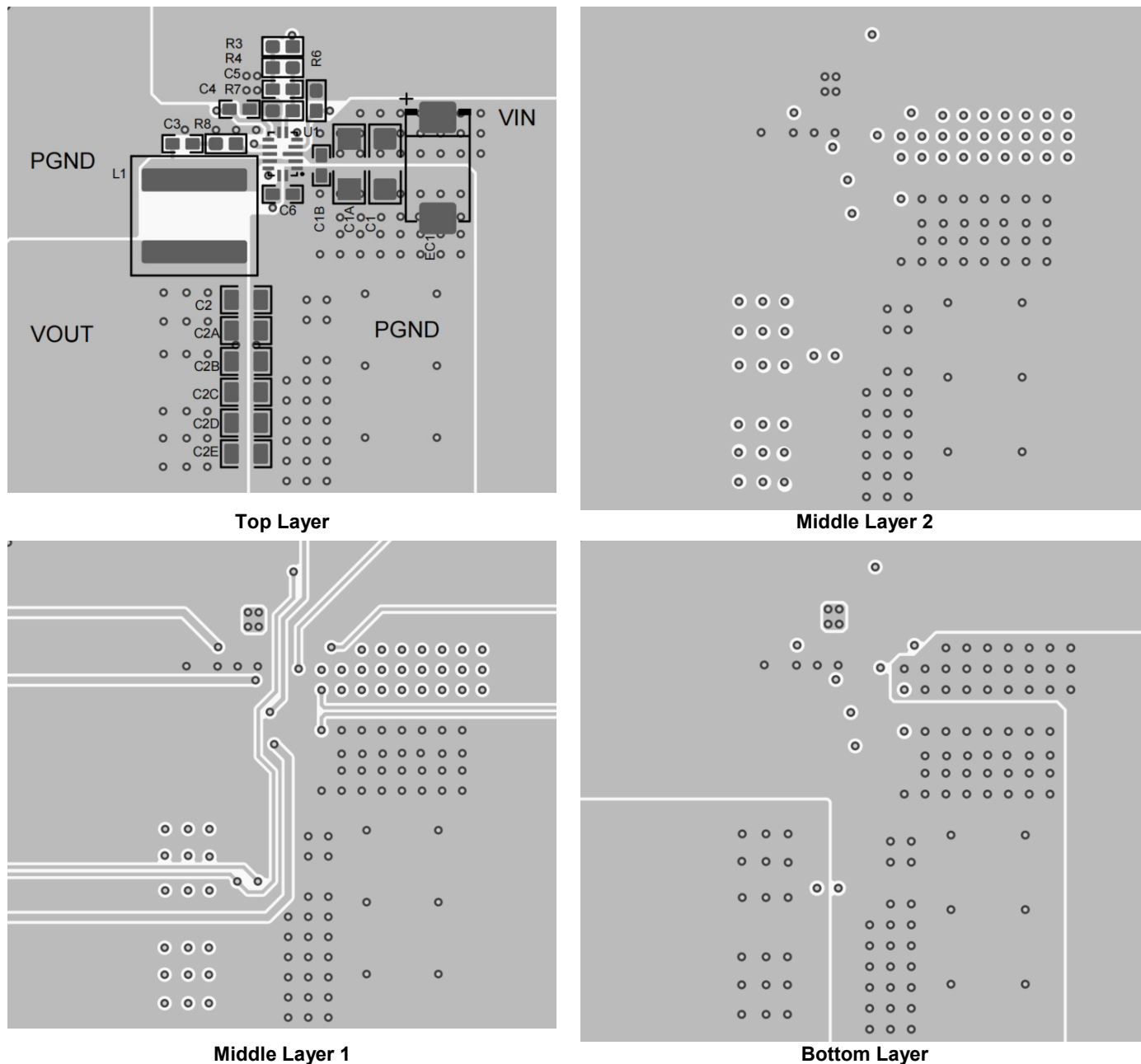
Figure 5. PCB Layout
