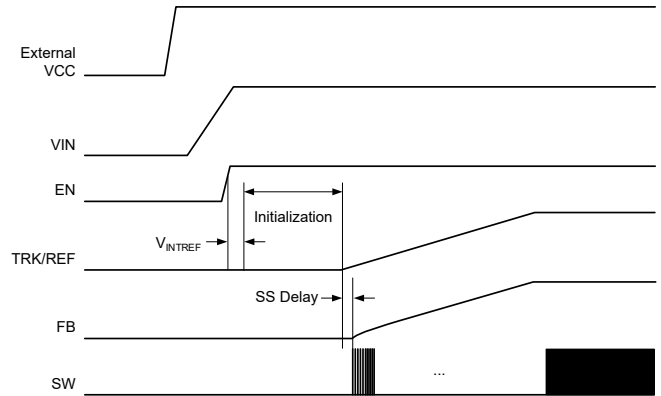
Figure 4. Power-up Sequence with External VCC
