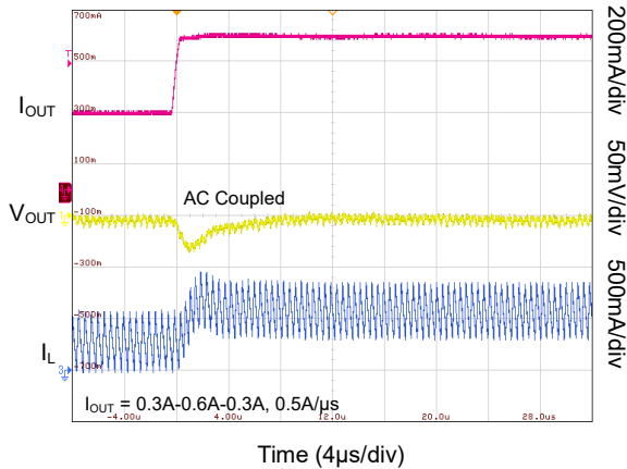
Load Transient Response in CCM, Rising Edge
