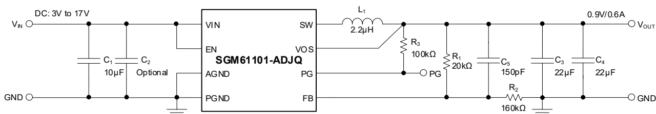
Figure 4. 0.9V Output Voltage Application of SGM61101-ADJQ
