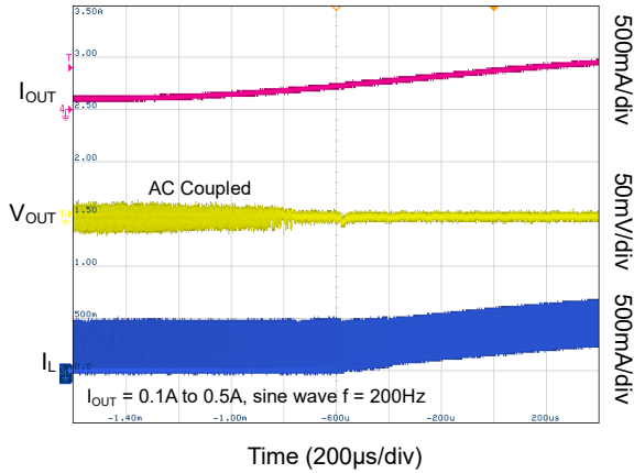
DCM to CCM Mode Transition
