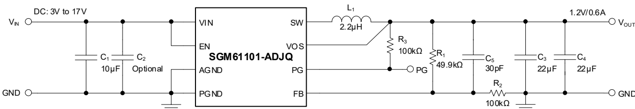
Figure 5. 1.2V Output Voltage Application of SGM61101-ADJQ
