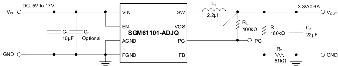
Figure 3. 3.3V Output Voltage Application of SGM61101-ADJQ
