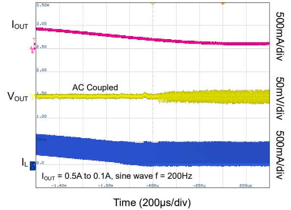
CCM to DCM Mode Transition
