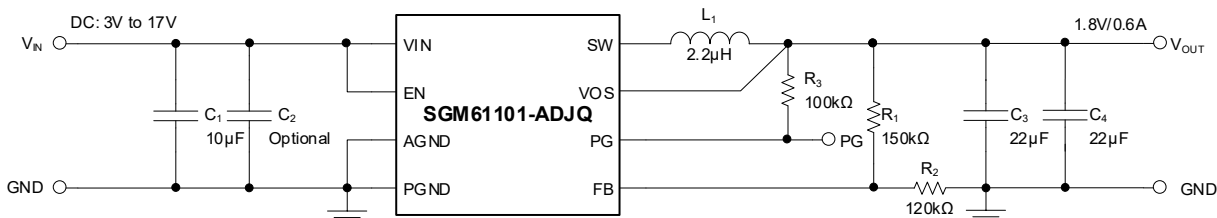
Figure 6. 1.8V Output Voltage Application of SGM61101-ADJQ
