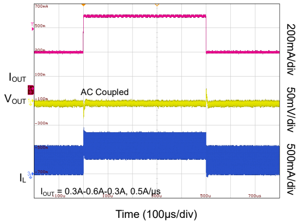
Load Transient Response in CCM
