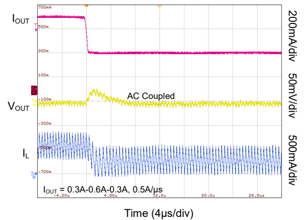
Load Transient Response in CCM, Falling Edge
