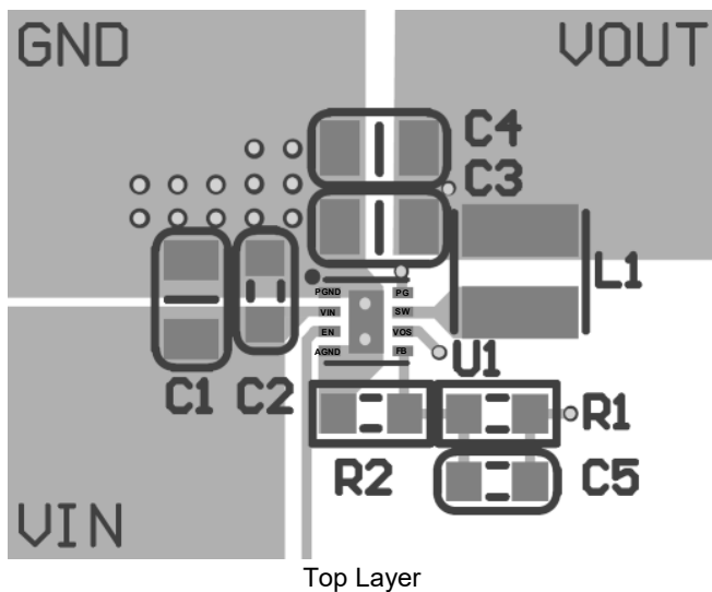
Figure 8. PCB Layout
