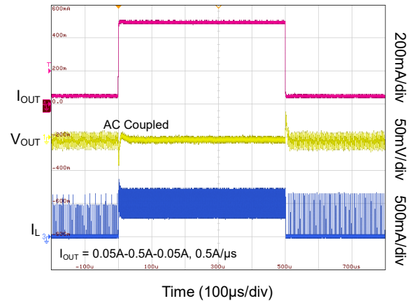
Load Transient Response from DCM to CCM
