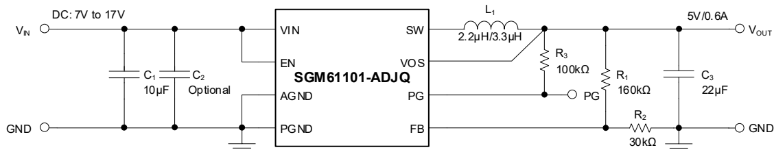
Figure 7. 5V Output Voltage Application of SGM61101-ADJQ
