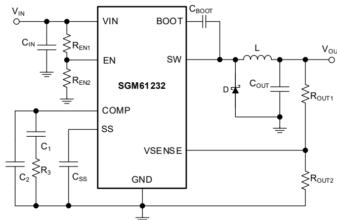
Figure 1. Simplified Schematic
