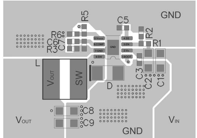
Figure 5. Top Layer
