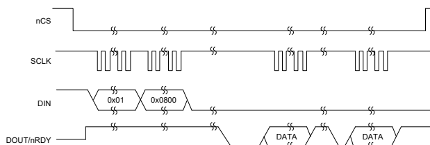
Figure 24. Continuous Read Configuration
