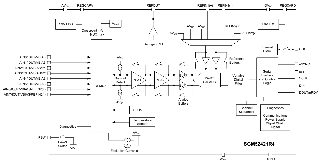
Figure 7. Block Diagram
