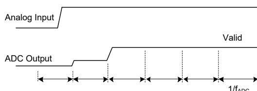
Figure 43. Step Change on the Analog Input, Sinc 4 + Sinc 1 Filter
