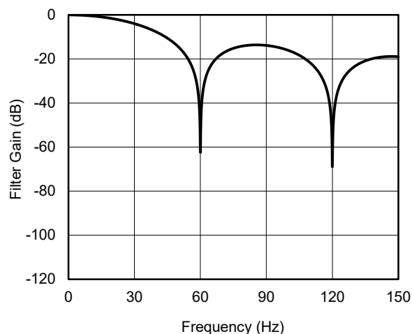
Figure 45. 60Hz Rejection
