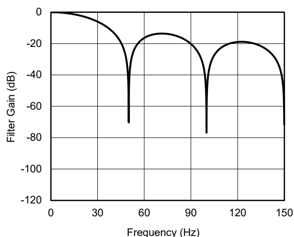
Figure 44. 50Hz Rejection
