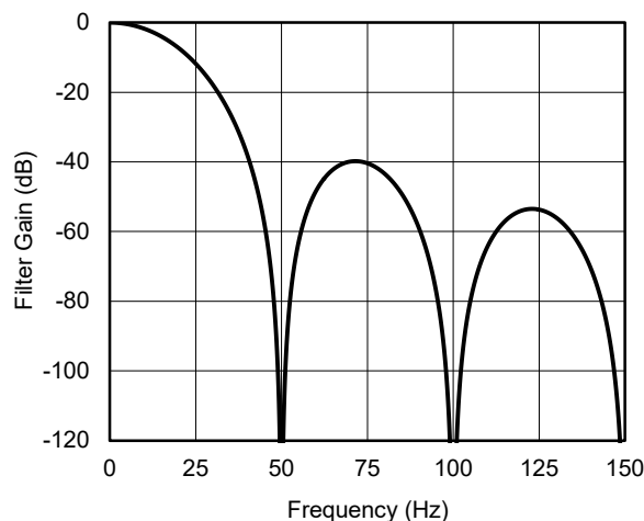
Figure 37. Sinc 3 Filter Response (50SPS with Zero Latency Disabled or 16.67SPS with Zero Latency Enabled)
