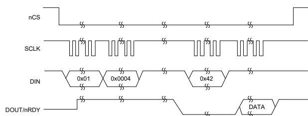
Figure 22. Single Conversion Configuration
