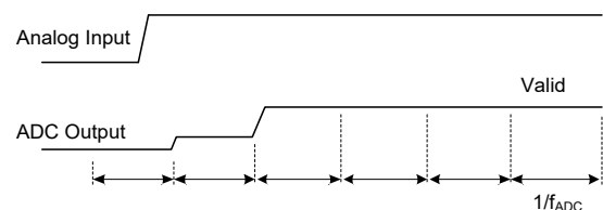
Figure 49. Step Change on the Analog Input, Sinc 3 + Sinc 1 Filter
