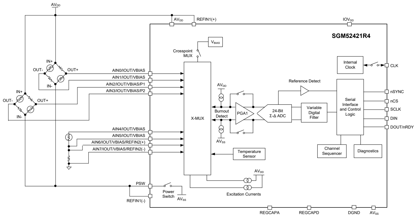
Figure 8. Basic Connection Diagram
