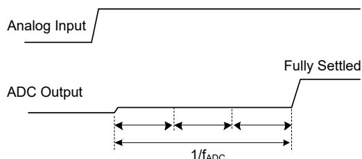
Figure 36. Sinc 3 Zero Latency Operation
