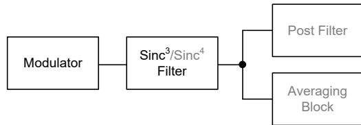
Figure 33. Sinc 3 Filter
