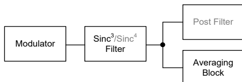
Figure 47. Fast Settling Mode, Sinc 3 + Sinc 1 Filter
