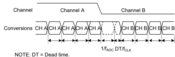
Figure 48. Fast Settling, Sinc 3 + Sinc 1 Filter
