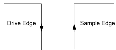
Figure 9. SPI Mode 3, SCLK Edges
