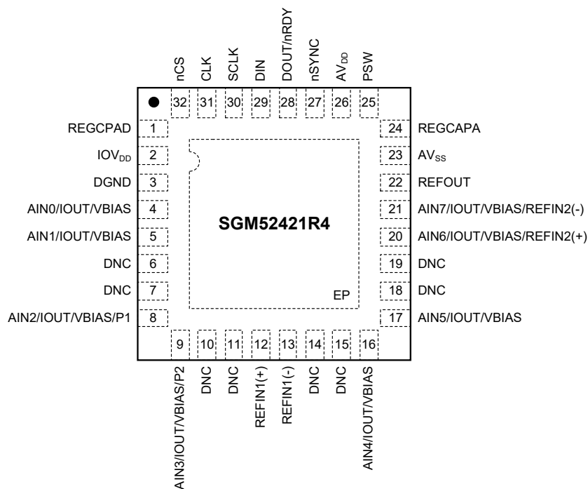
TQFN-5x5-32IL
