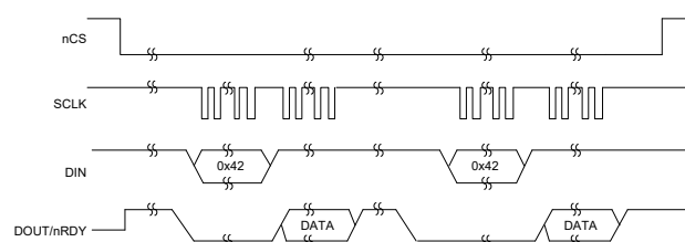
Figure 23. Continuous Conversion Configuration
