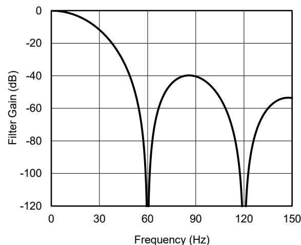
Figure 38. Sinc 3 Filter Response (60SPS with Zero Latency Disabled or 20SPS with Zero Latency Enabled)
