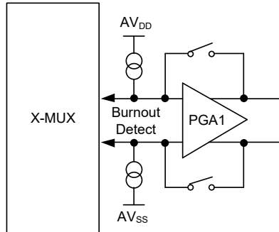
Figure 68. Burnout Currents
