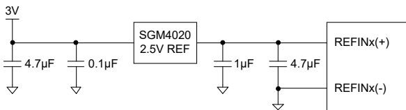
Figure 20. Reference Voltage Wiring for SGM52421R4
