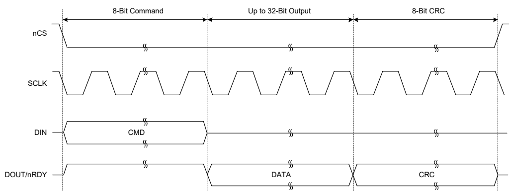
Figure 67. SPI Read Transaction with CRC
