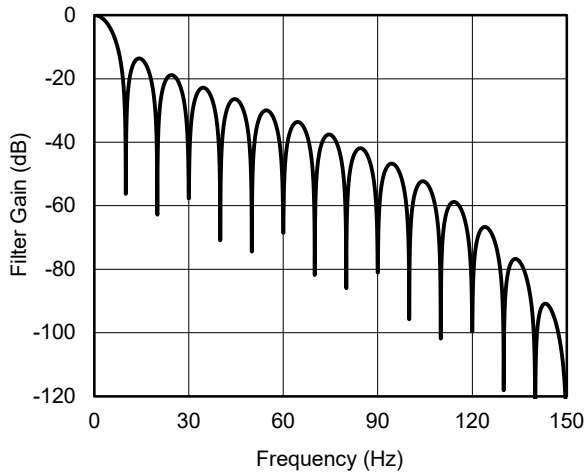
Figure 46. Simultaneous 50Hz and 60Hz Rejection
