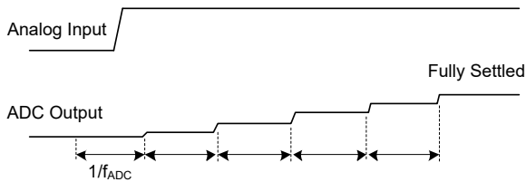
Figure 27. Asynchronous Step Change in the Analog Input
