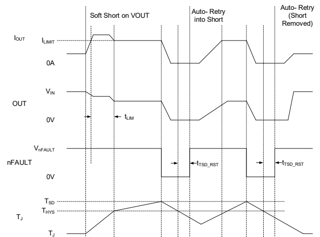
Figure 5. SGM2537-xR/xRD/xRN Over-Current Response (Auto-Retry)
