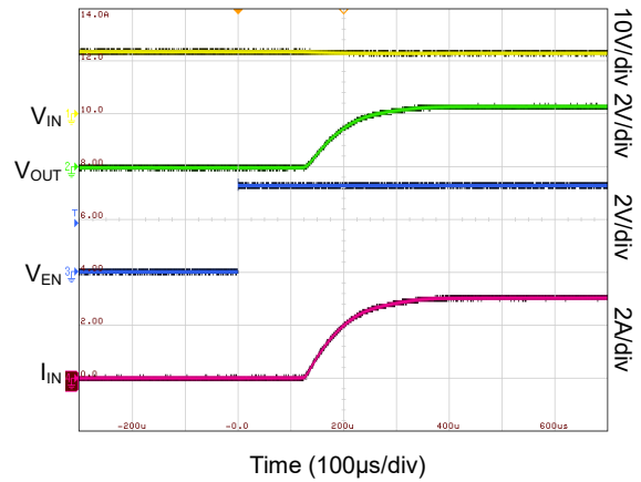
Figure 15. Output Ramp with 4Ω Load at Start-Up
