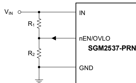
Figure 3. Over-Voltage Lockout
