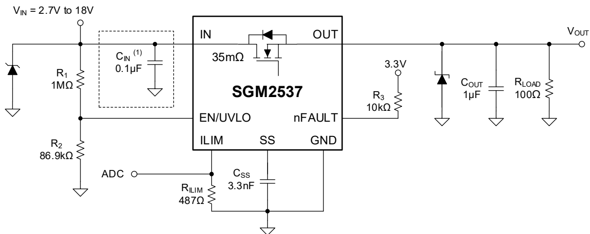
Figure 21 shows a circuit implementation with optional protection components.
