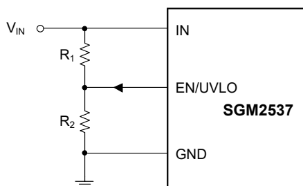
Figure 2. Under-Voltage Lockout
