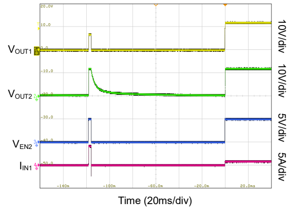
Figure 12. SGM2537-13.7R Self-Controlled Mode Response with Overload on OUT1 Followed by Recovery with Fault Removed
