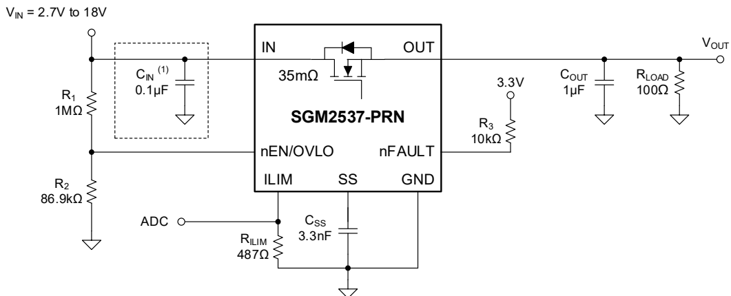
Figure 19. Circuit Implementation for Over-Voltage Lockout Using SGM2537-PRN
