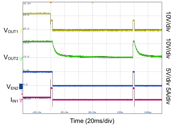
Figure 11. SGM2537-13.7R Self-Controlled Mode Response with Overload Fault on OUT1 Followed by Auto-Retry with Persistent Fault
