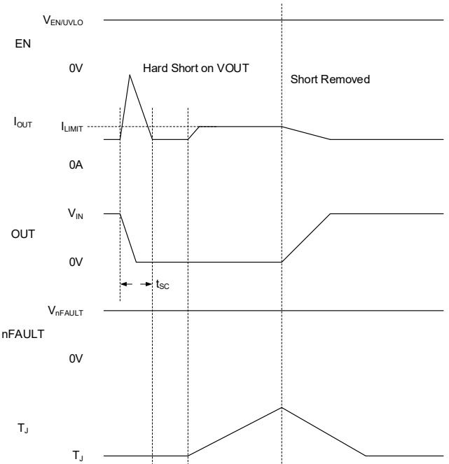
Figure 7. SGM2537 Short-Circuit Response
