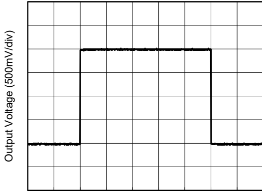
Time (100µs/div)
